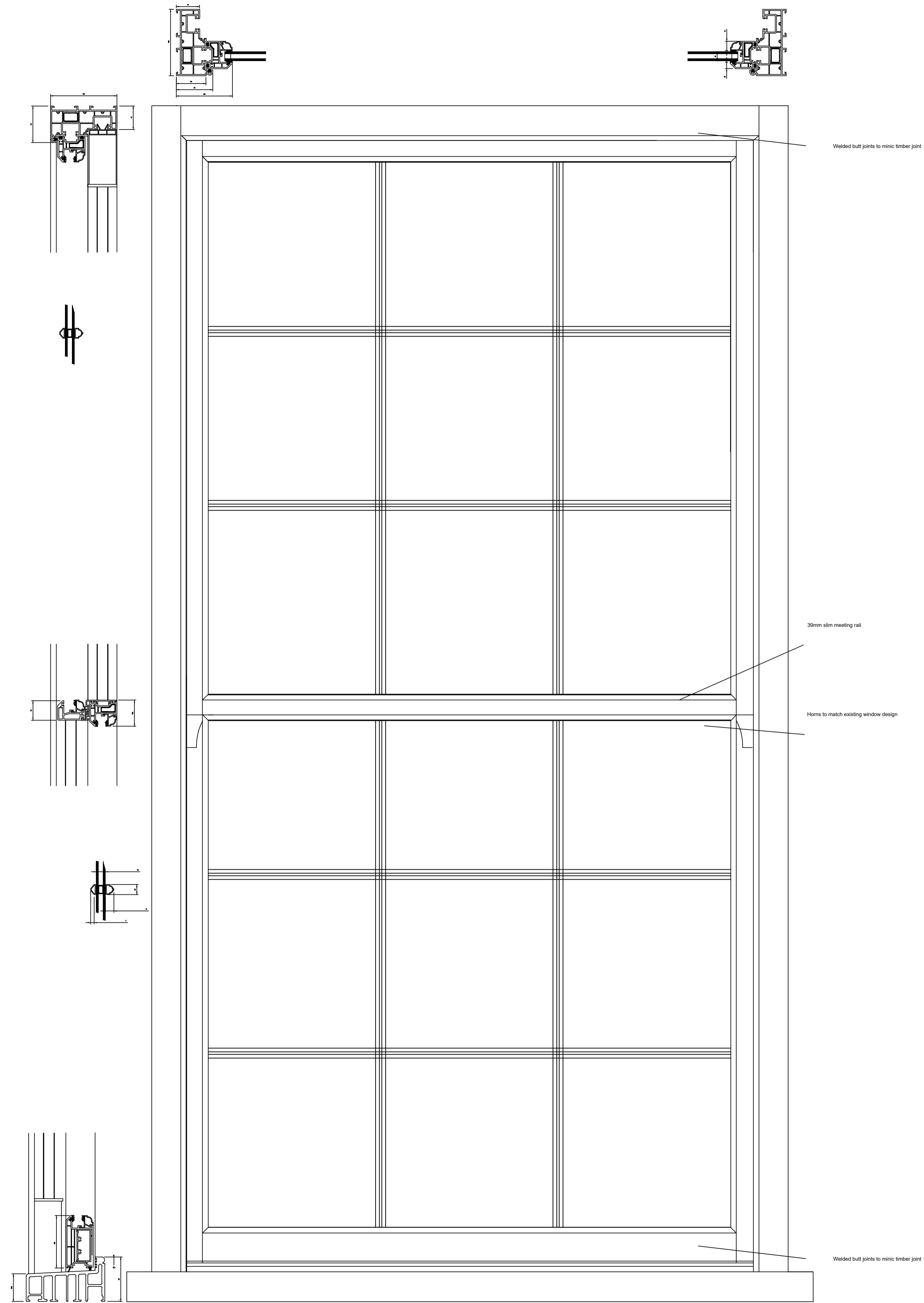
Proposed white Heritage Style uPVC 1st Floor Window
