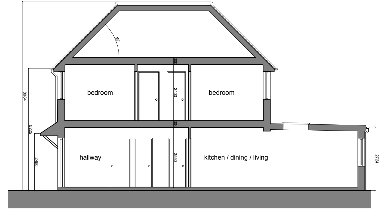
PROPOSED SECTION
