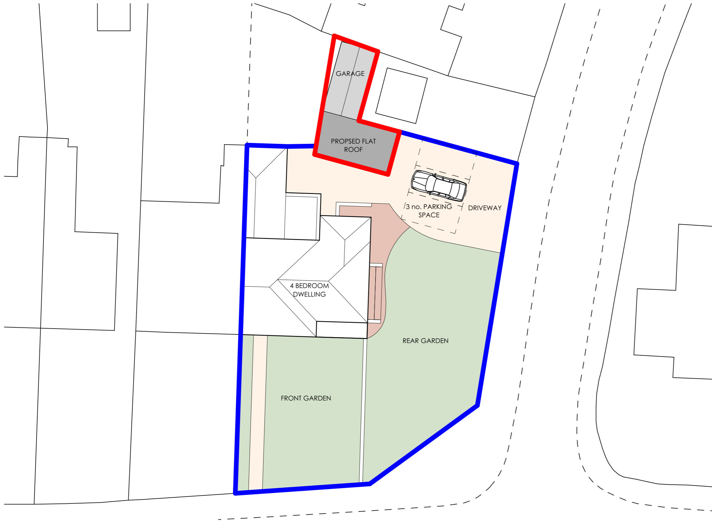
01 Proposed Site Plan 1:200
