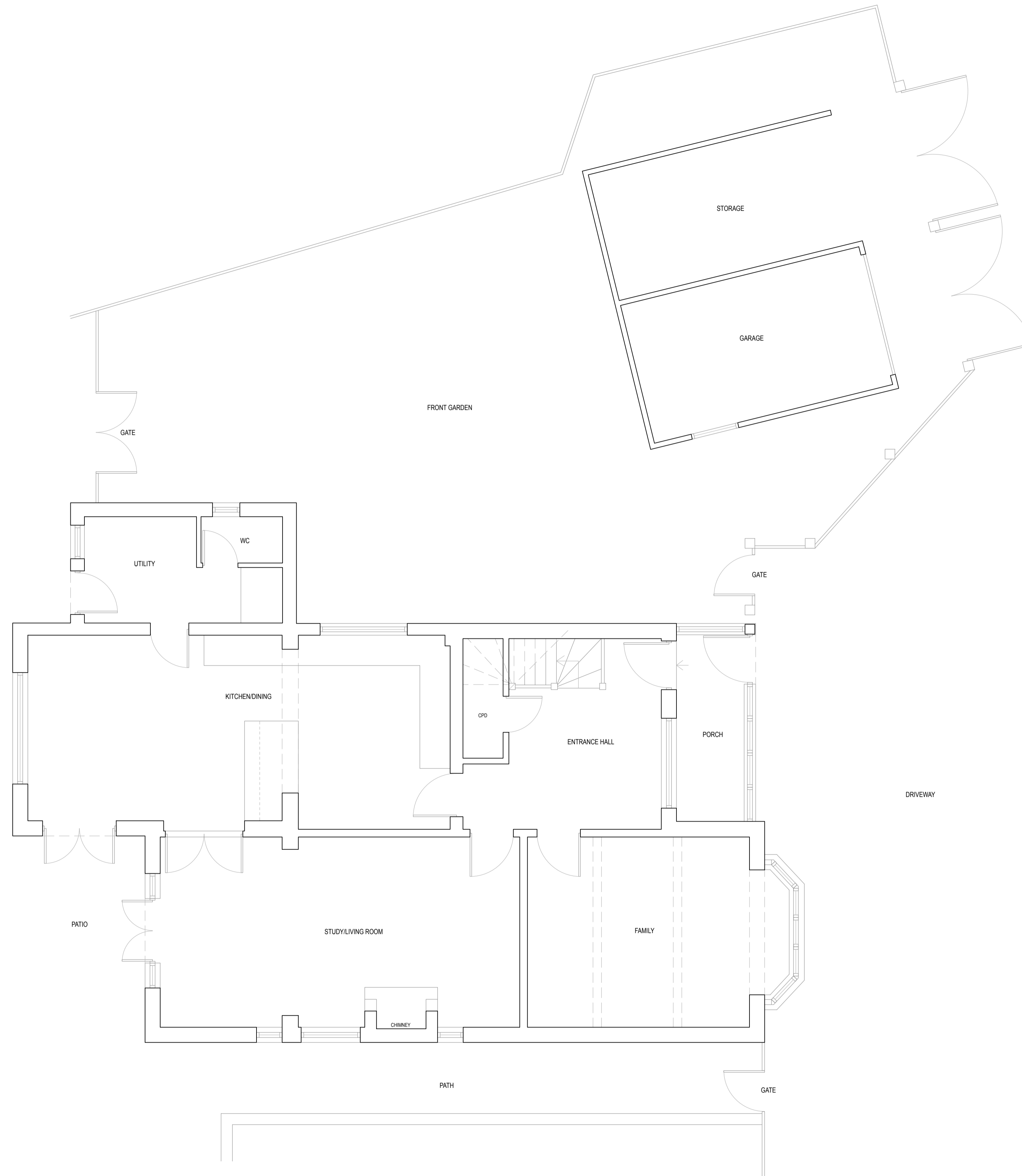
EXISTING GROUND FLOOR PLAN Scale 1:50
