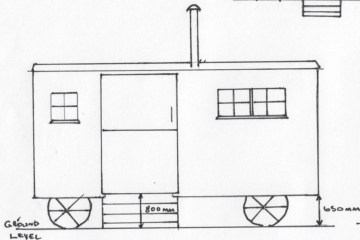
EASTERN ELEVATION
