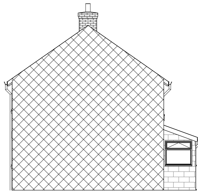
3 North East Elevation 1 : 100
