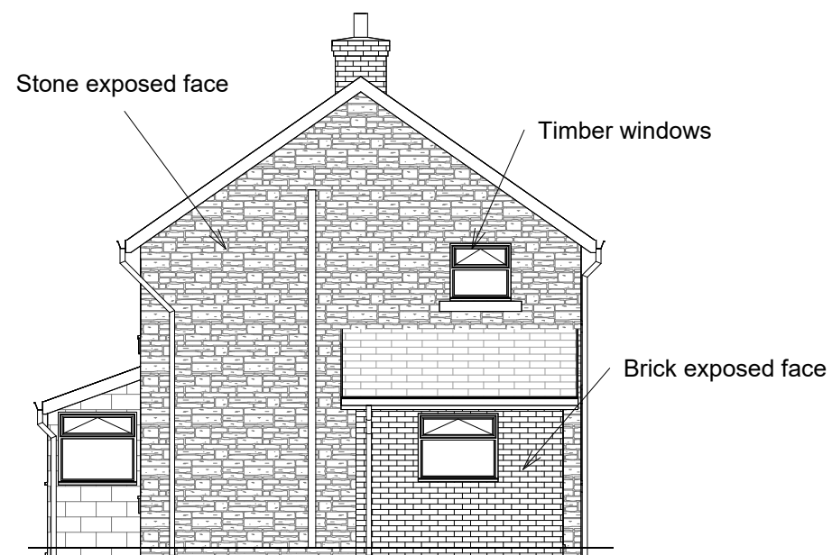
6 South West Elevation 1 : 100
