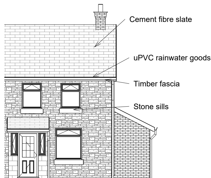
4 North West Elevation 1 : 100
