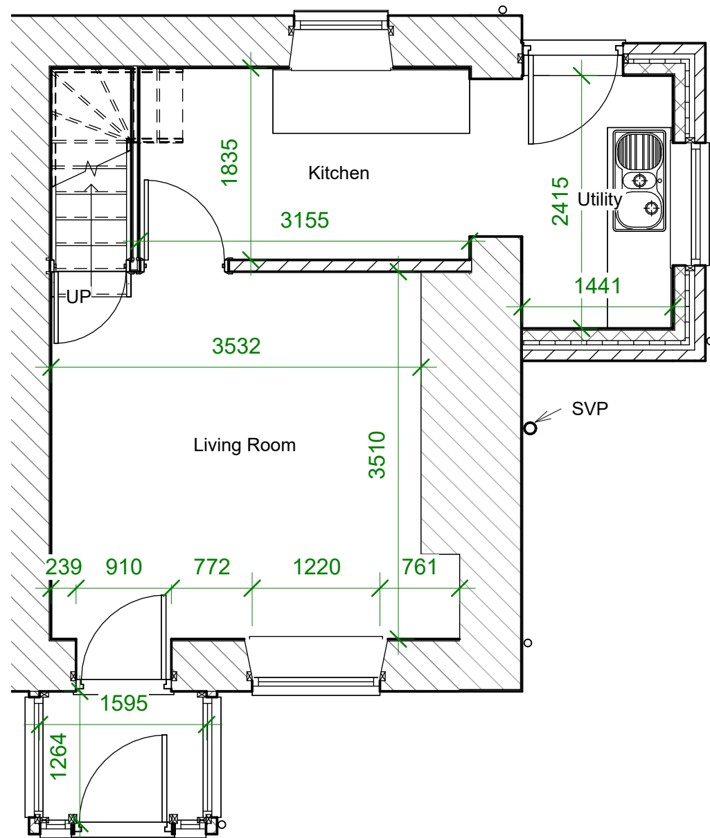
1 Ground Floor 1 : 50
