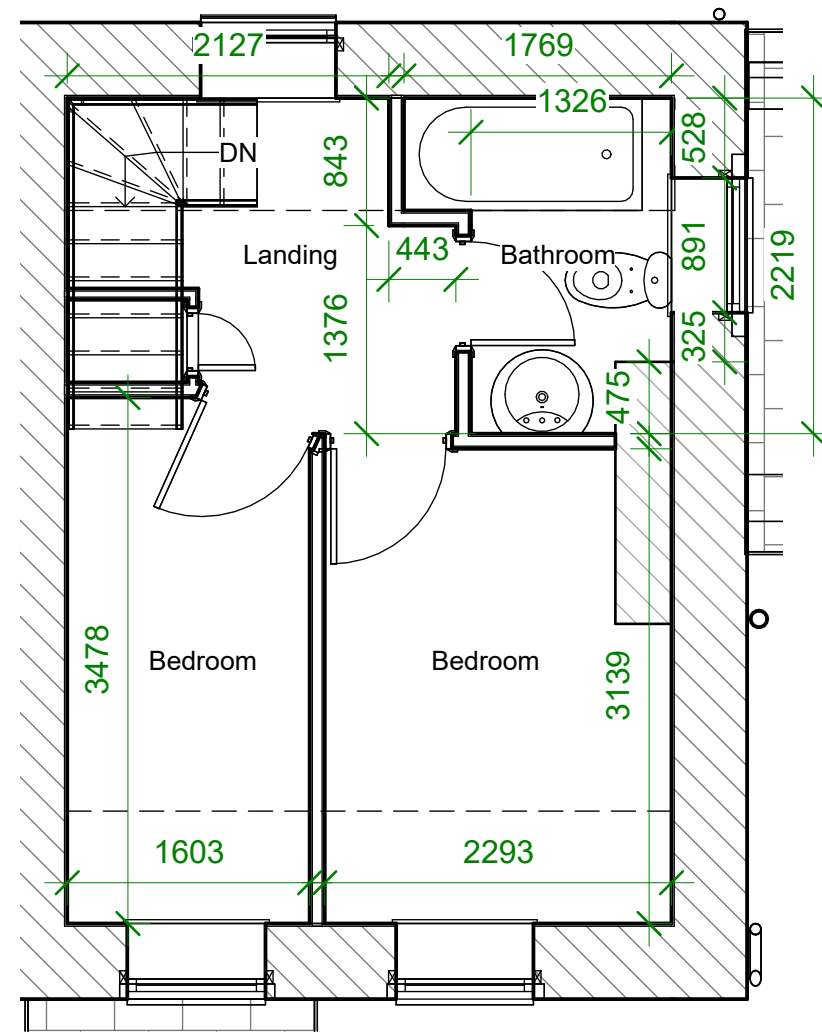
2 First Floor 1 : 50
