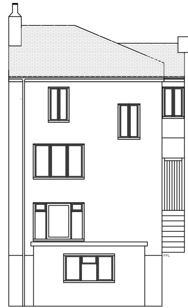
Existing North East elevation
