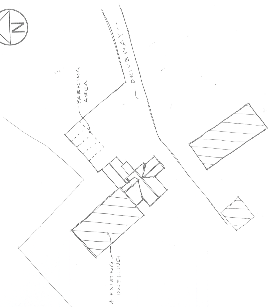
BLOCK PLAN ~ 1:500
