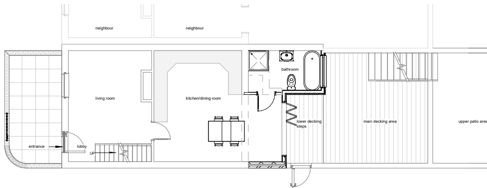
Proposed Ground Floor
