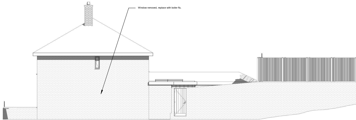
Proposed Elevation-Right side
