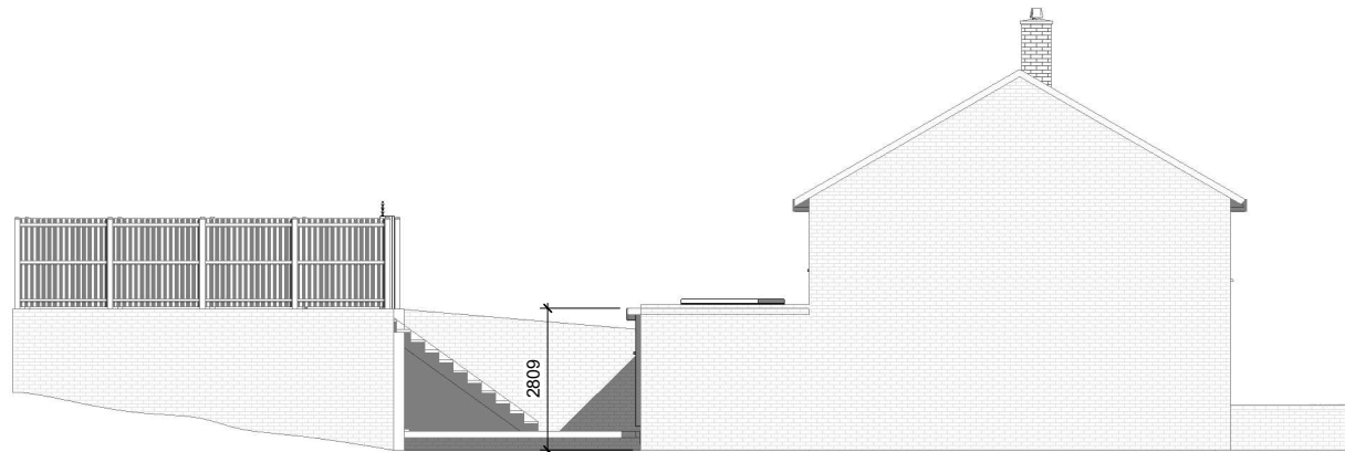
Proposed Elevation-Left side
