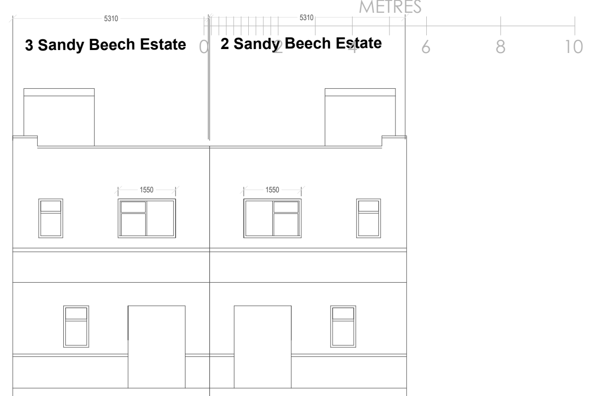
Existing Rear Elevation (North)
