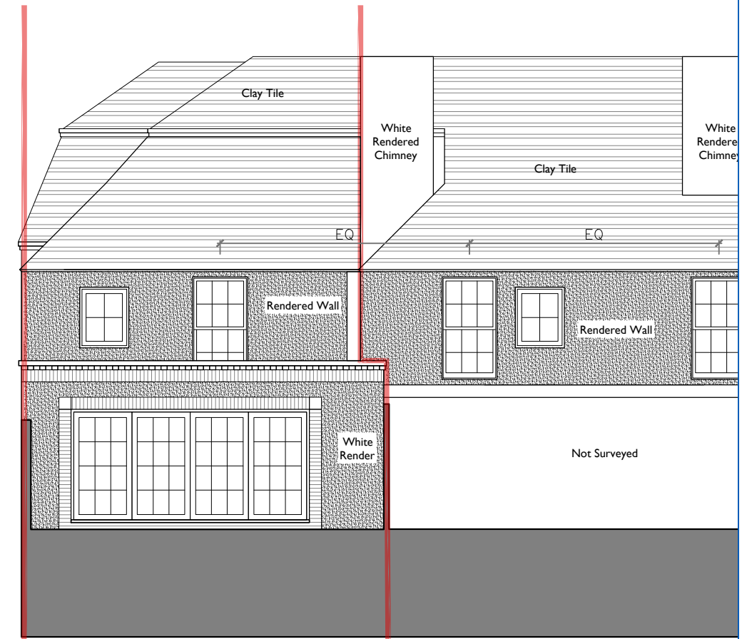
West Elevation 1:100
