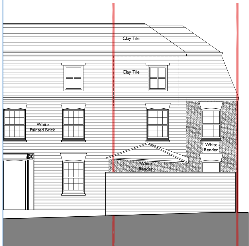
East Elevation (Inc boundary wall) 1:100
