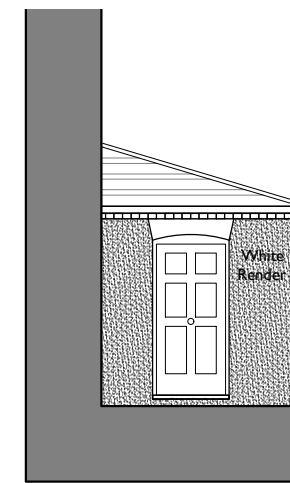
South Elevation Porch Entrance Lobby 1:100
