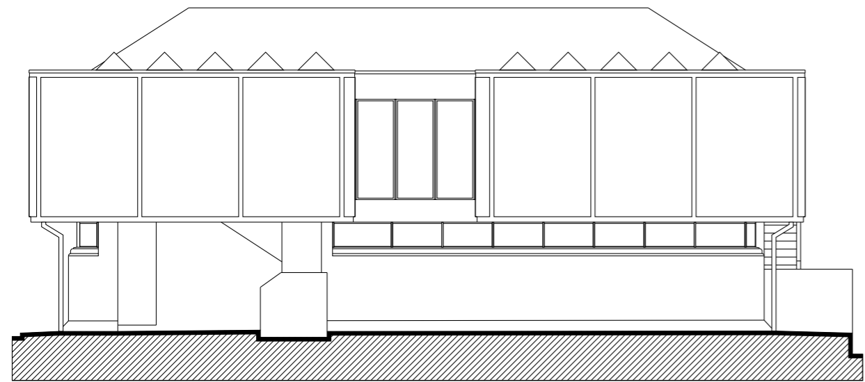
REAR ELEVATION - SOUTHEAST
