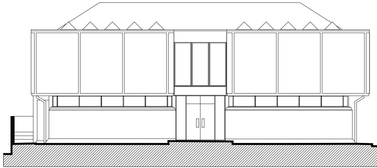
FRONT ELEVATION - NORTHWEST
