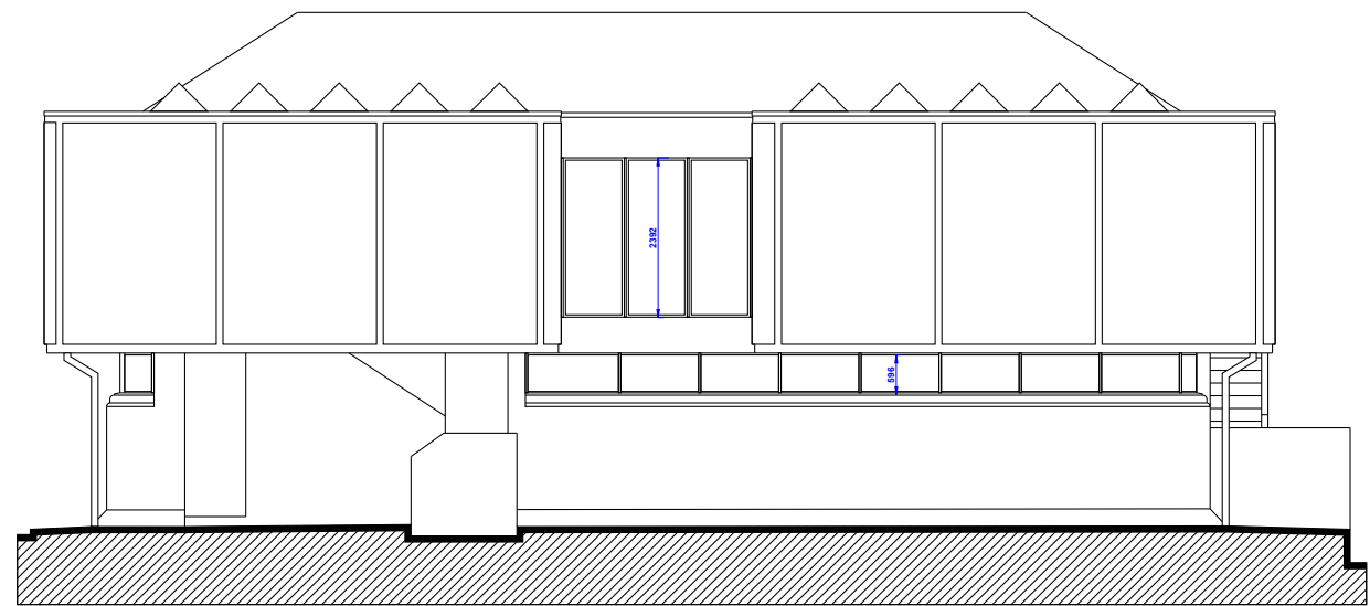
Datum 72.50m REAR ELEVATION - SOUTHEAST
