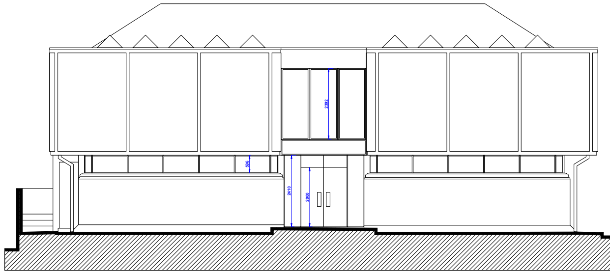
Datum 72.50m FRONT ELEVATION - NORTHWEST
