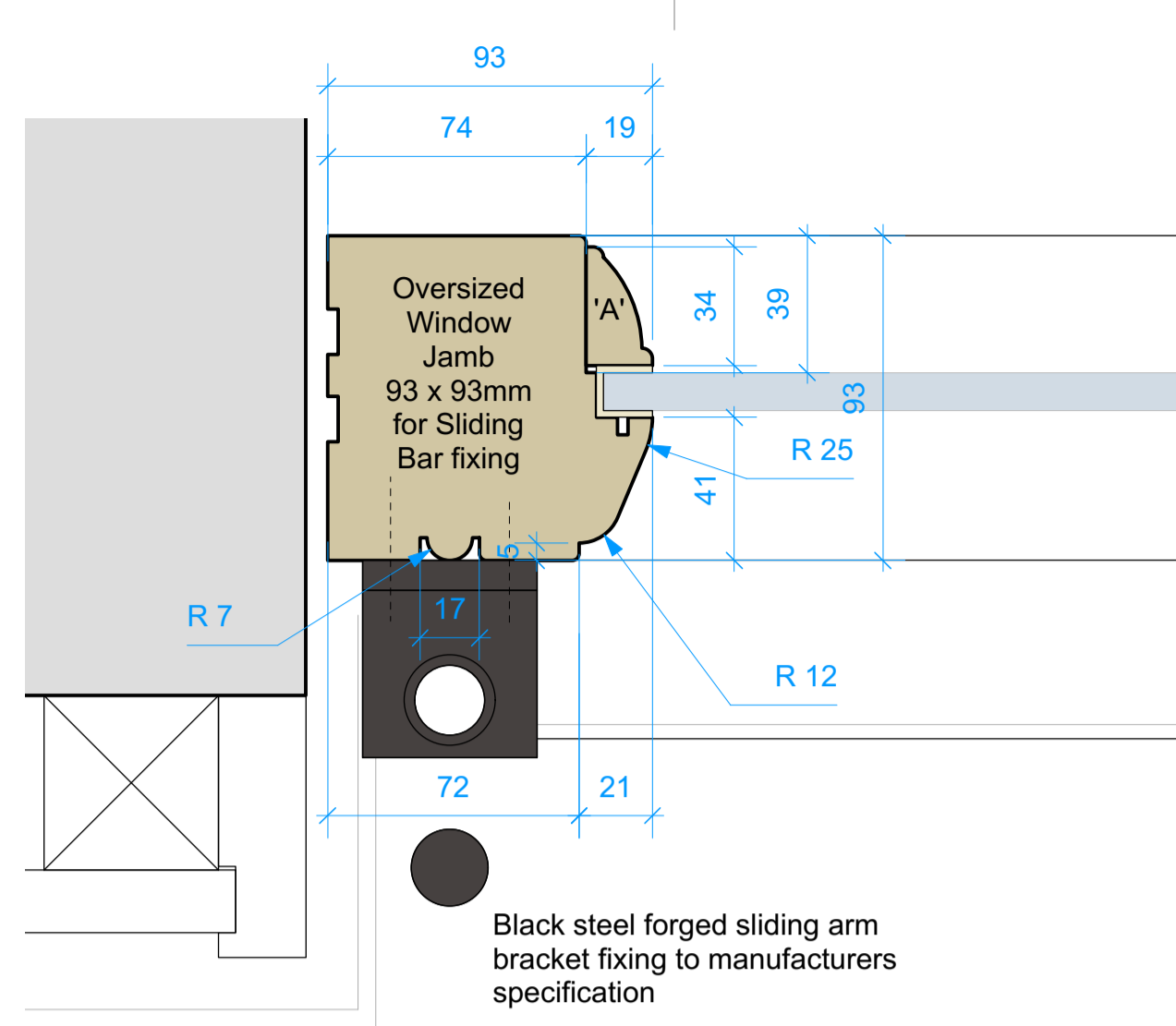
'LHS' WINDOW JAMB - PLAN VIEW
