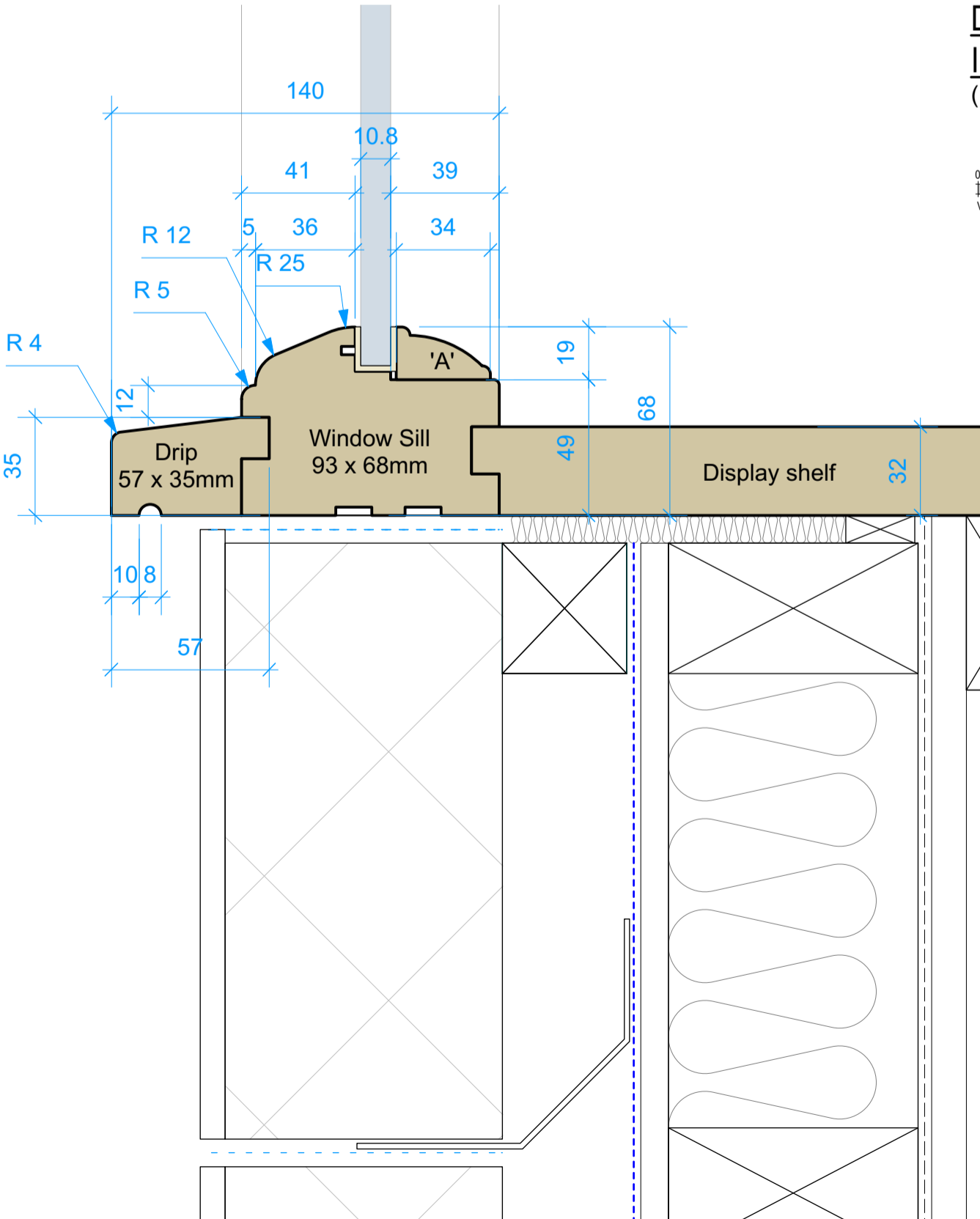
WINDOW SECTION
