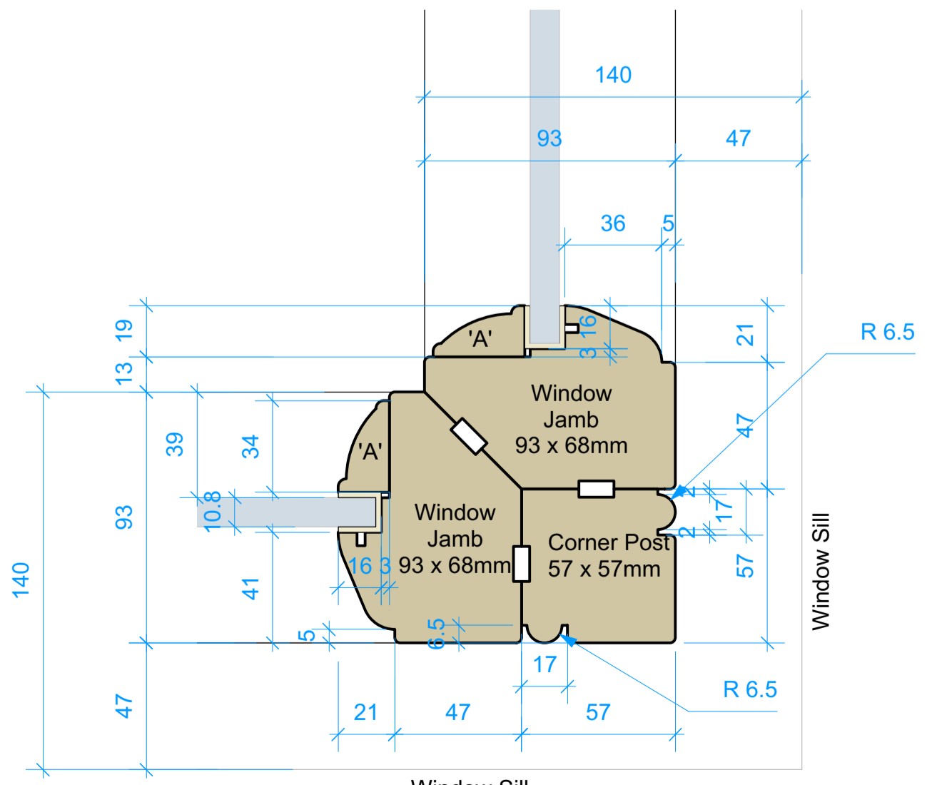
LHS WINDOW JAMB TO OUTER CORNER POST - PLAN VIEW
