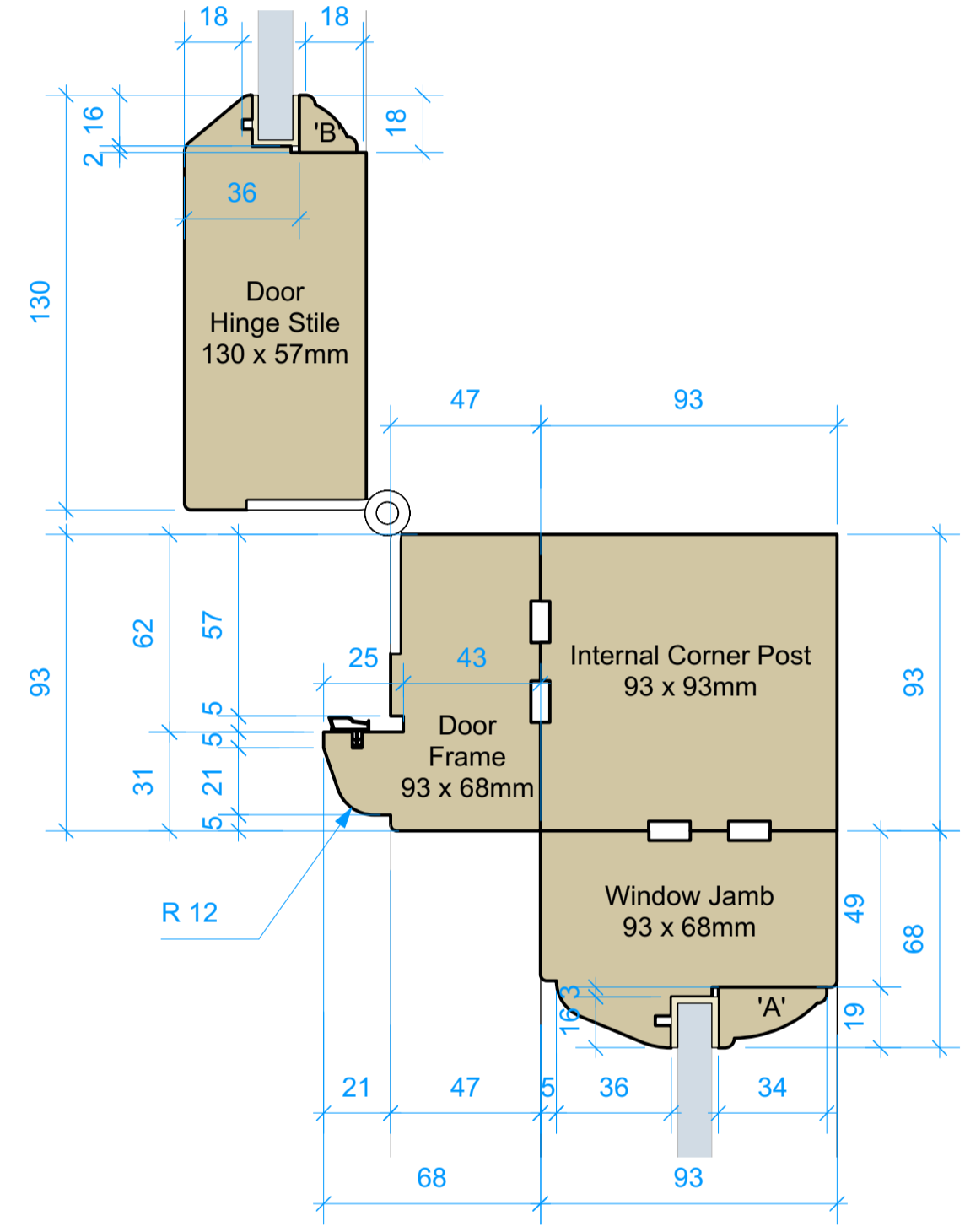
DOOR FRAME & WINDOW JAMB TO 'RHS' INTERNAL CORNER POST - PLAN VIEW (Door leaf shown open)
