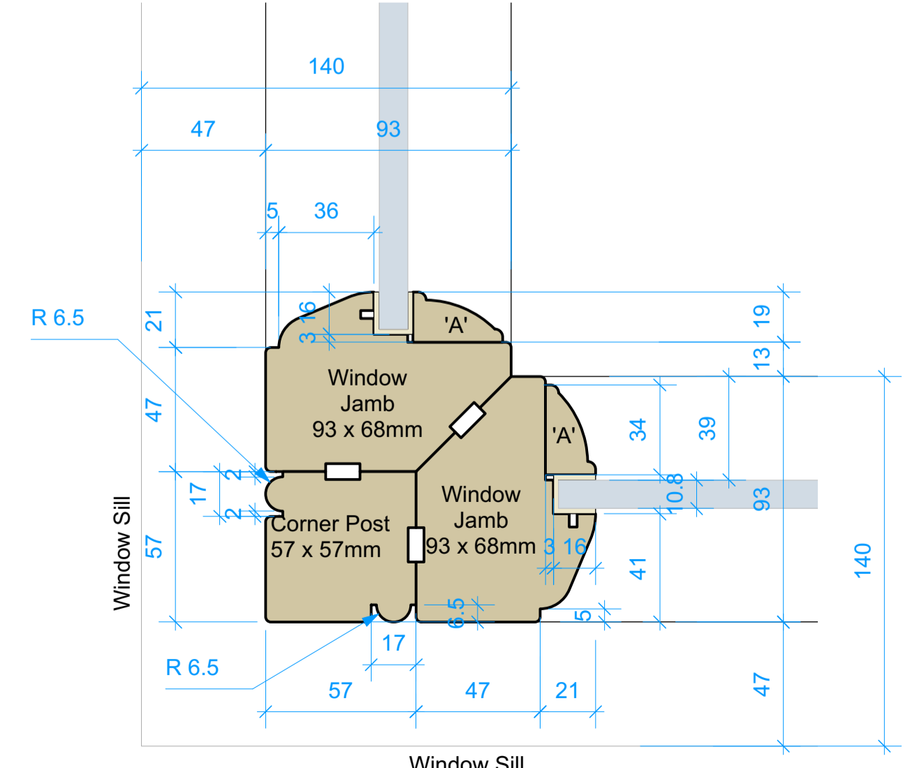
'RHS' WINDOW JAMB TO OUTER CORNER POST - PLAN VIEW
