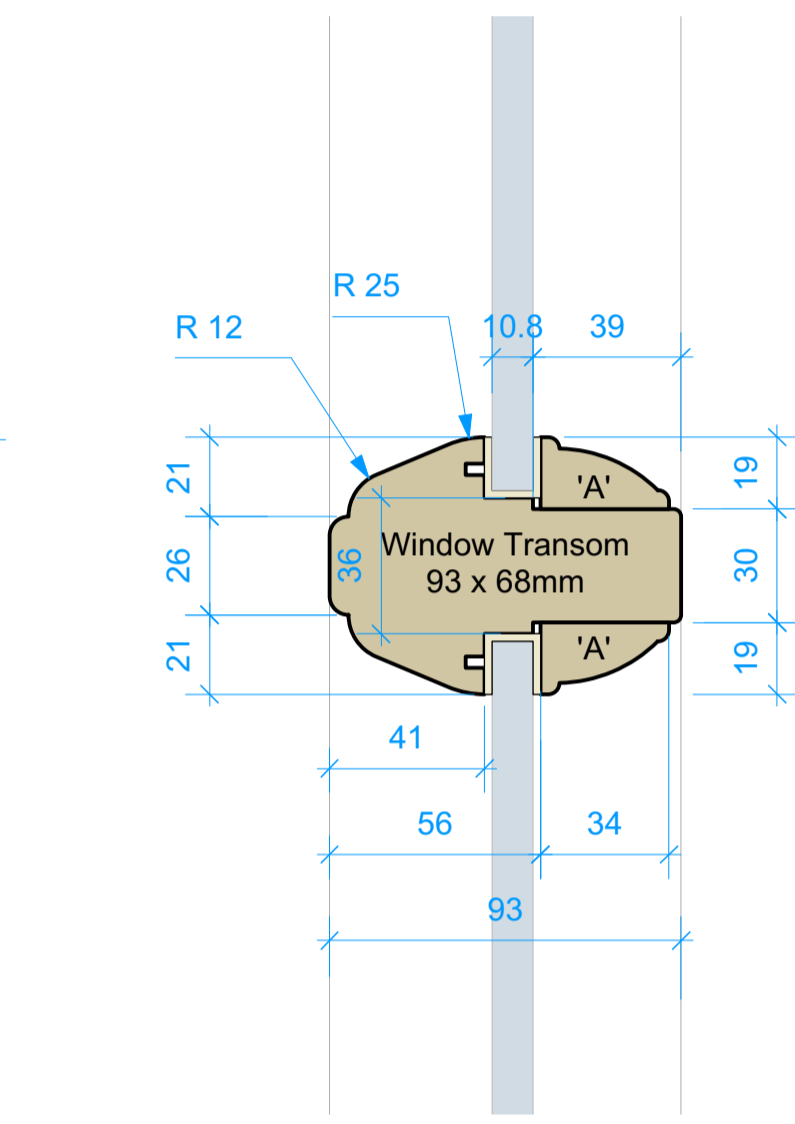
Direct glazed frame internally beaded
