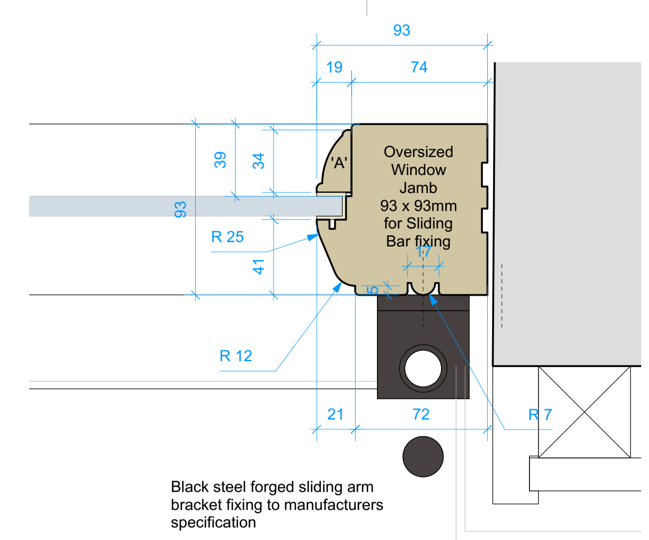
'RHS' WINDOW JAMB - PLAN VIEW
