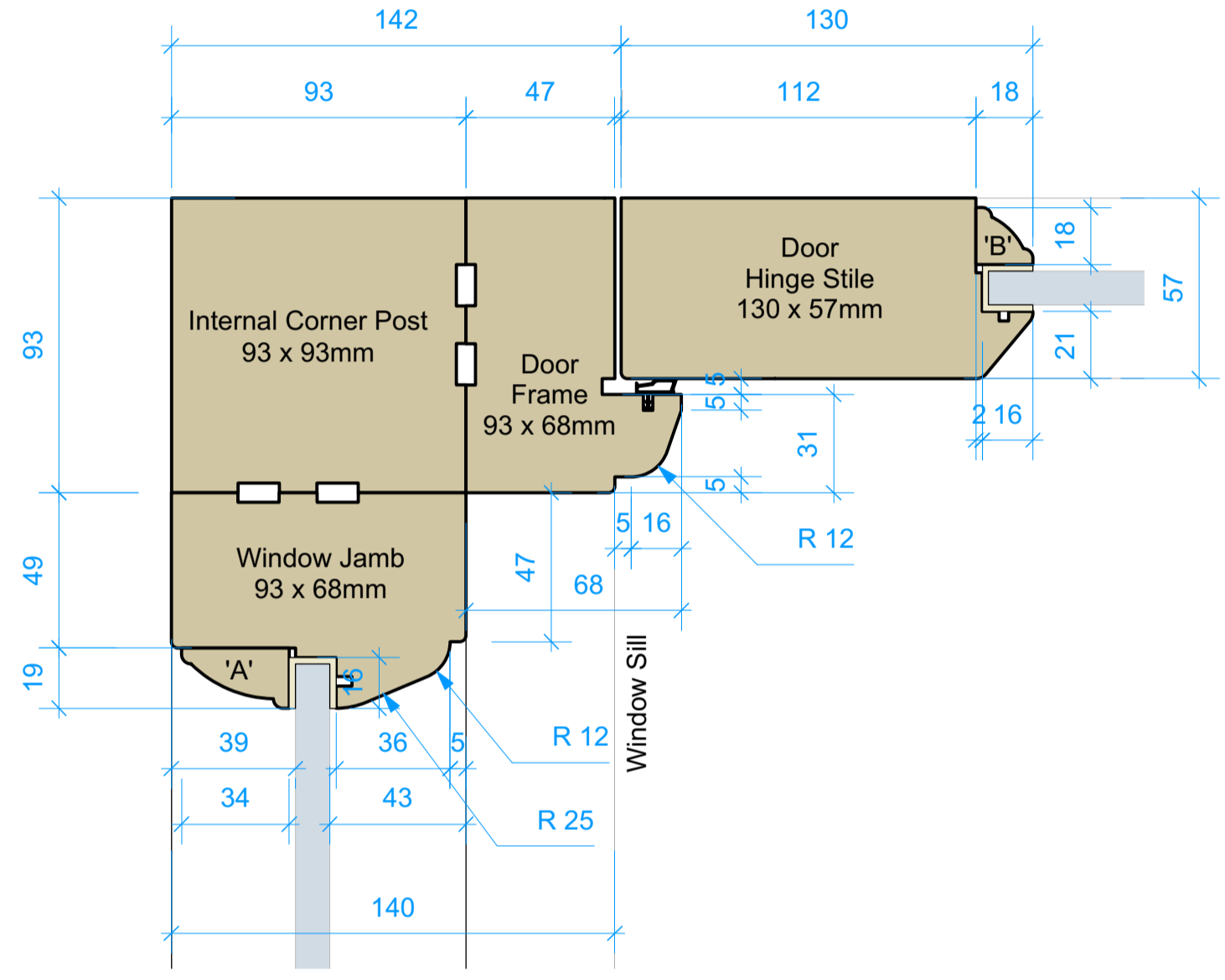
DOOR FRAME & WINDOW JAMB TO 'LHS' INTERNAL CORNER POST - PLAN VIEW (Door leaf shown closed)
