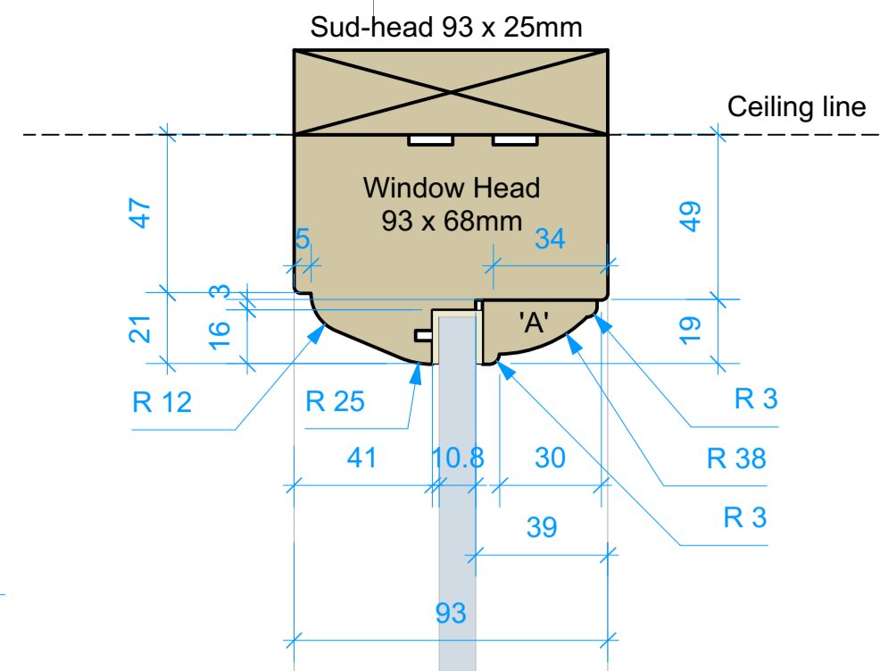
Direct glazed fanlight head above door and display windows internally beaded
