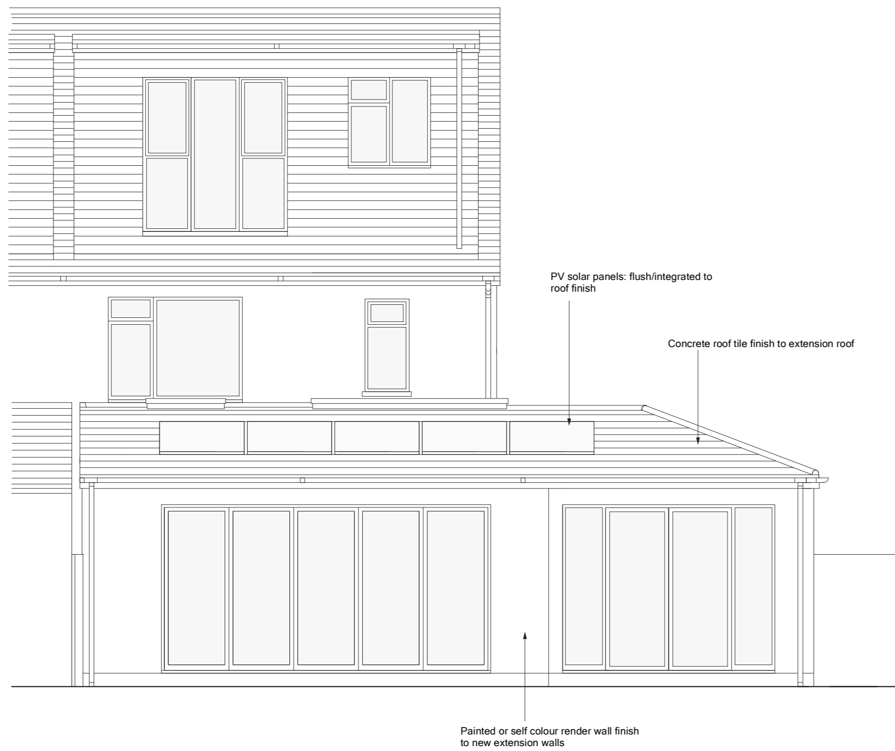
Proposed Rear Elevation scale 1:50 @ A2
