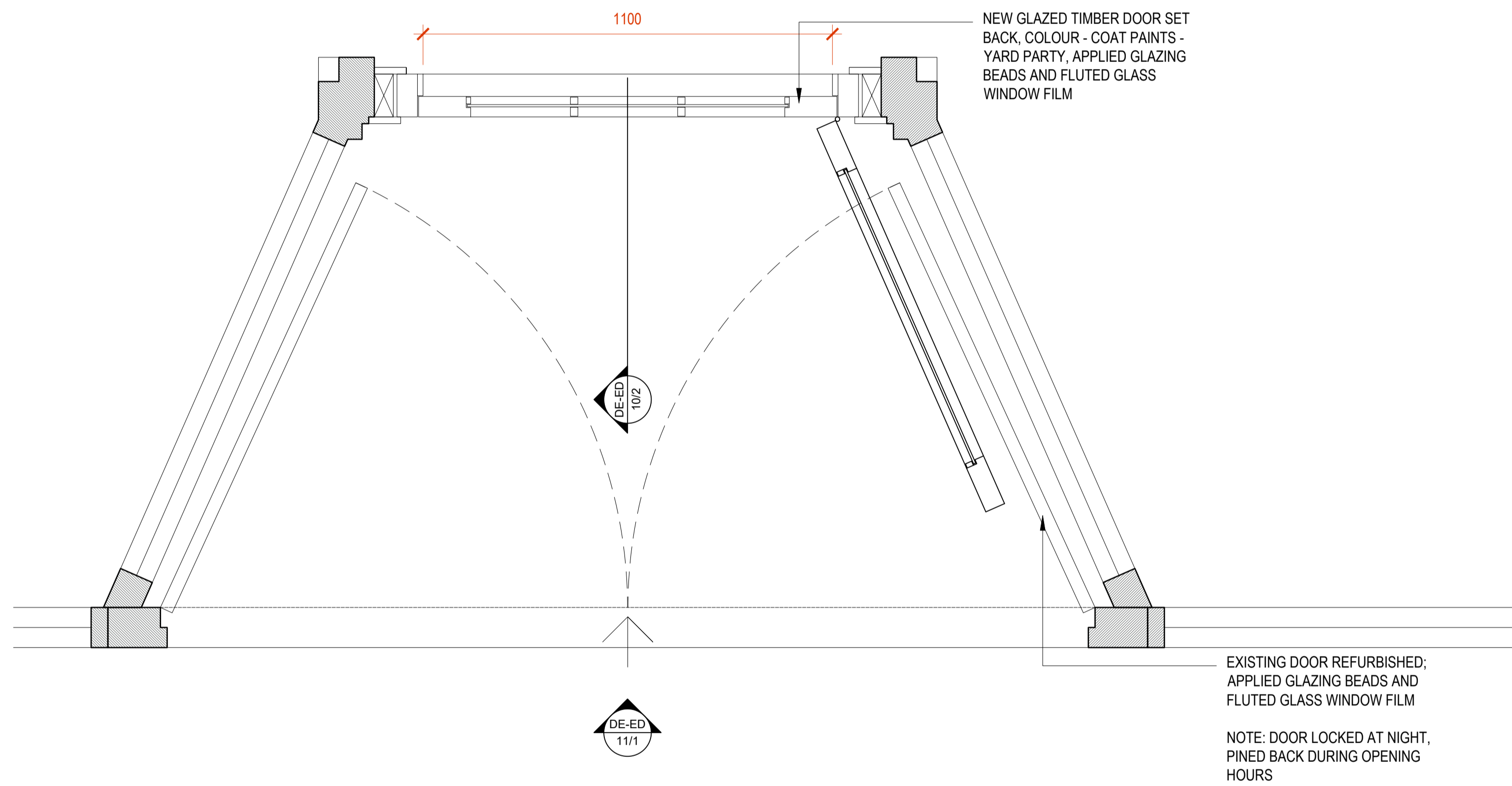
1 PLAN - ENTRANCE DOOR 1:10 @ A1
