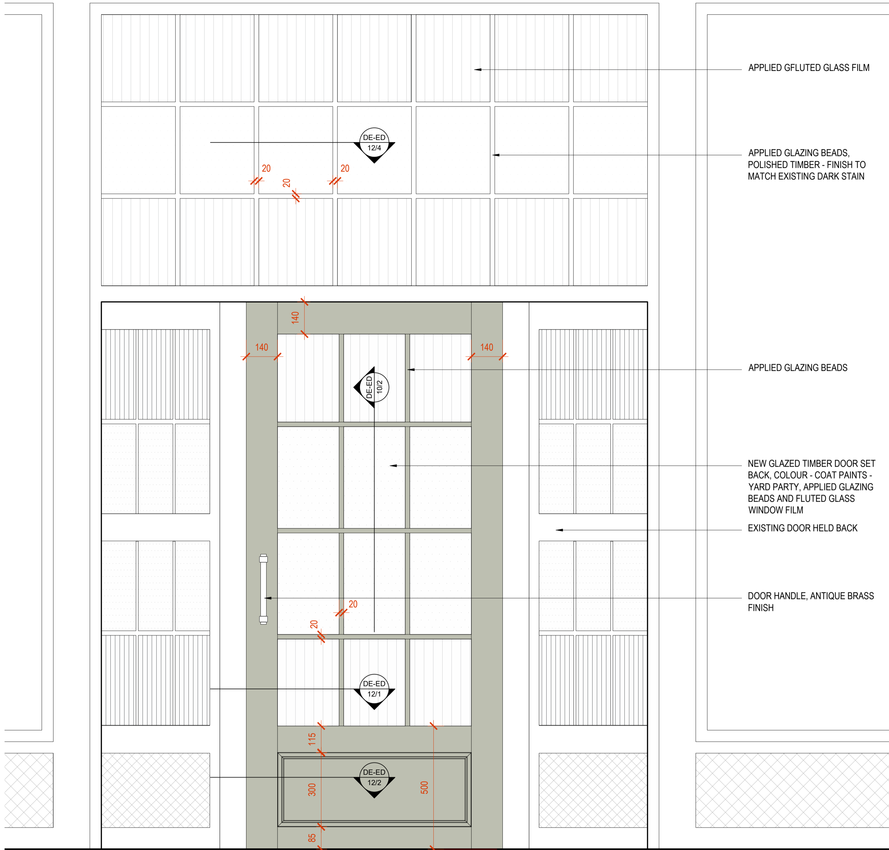
1 ELEVATION - EXISTING DOOR IN OPEN POSITION 1:10 @ A1
