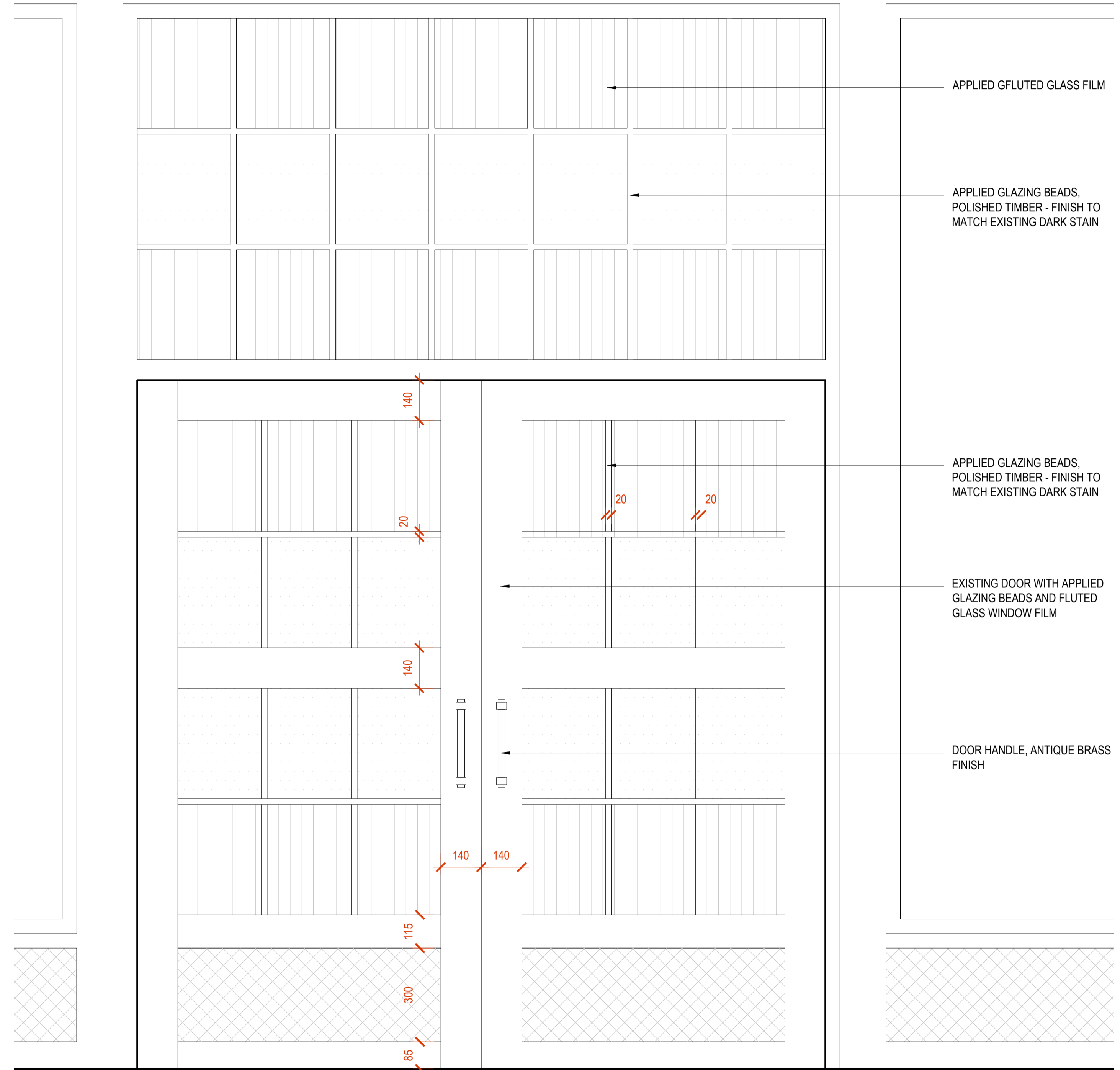
2 ELEVATION - EXISTING DOOR IN CLOSED POSITION 1:10 @ A1
