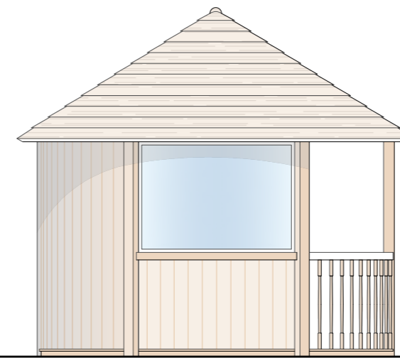
PROPOSED GAZEBO FLANK ELEVATION
