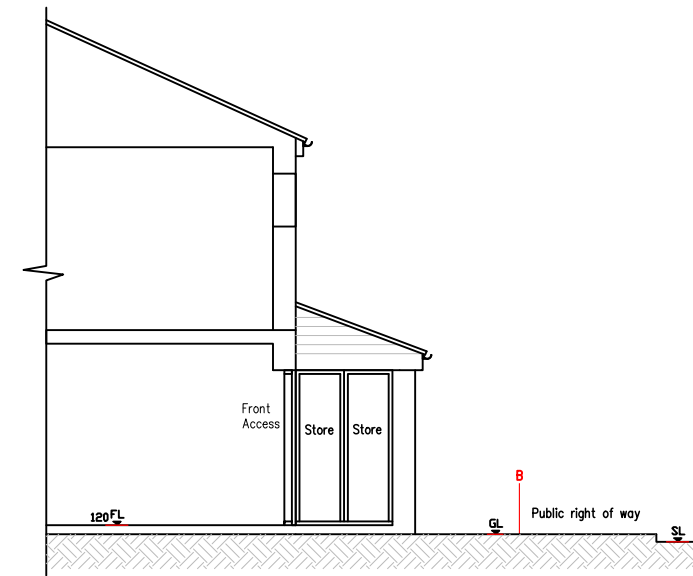
EXISTING SECTIONAL ELE. 'AA'
