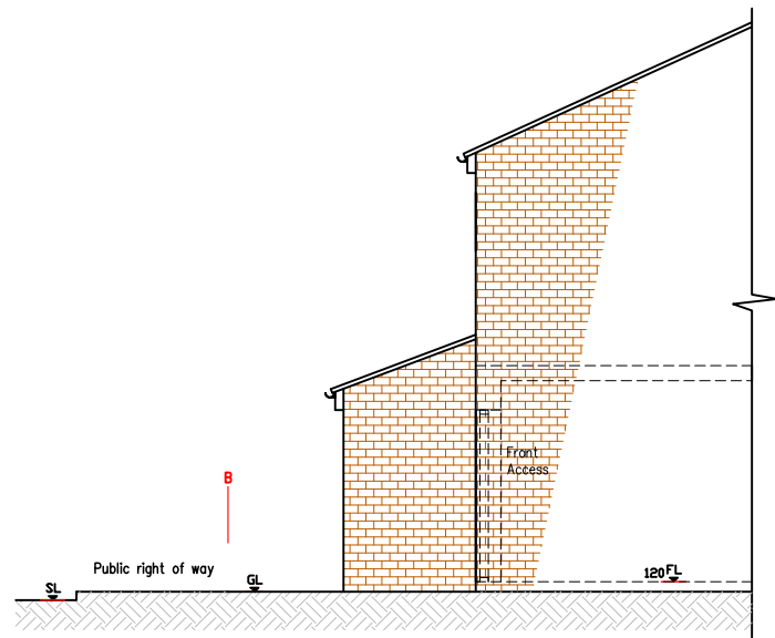
EXISTING END ELEVATION B
