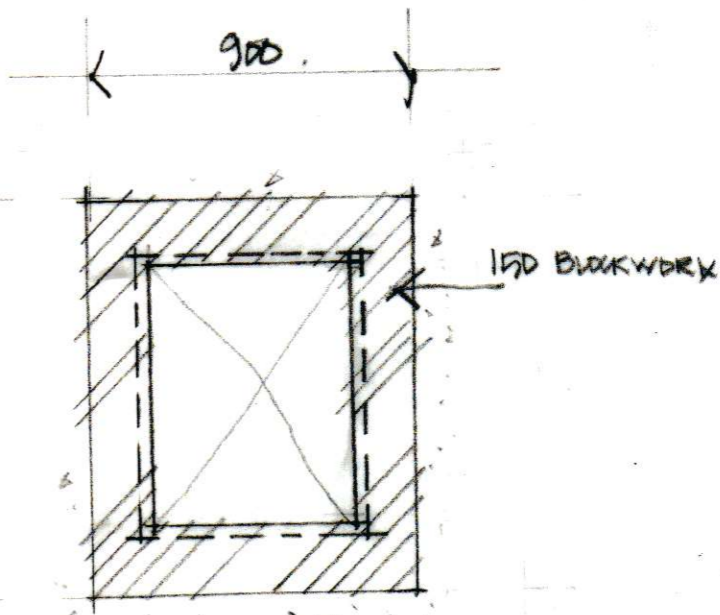
FOUNDATION PLAN 1:20
