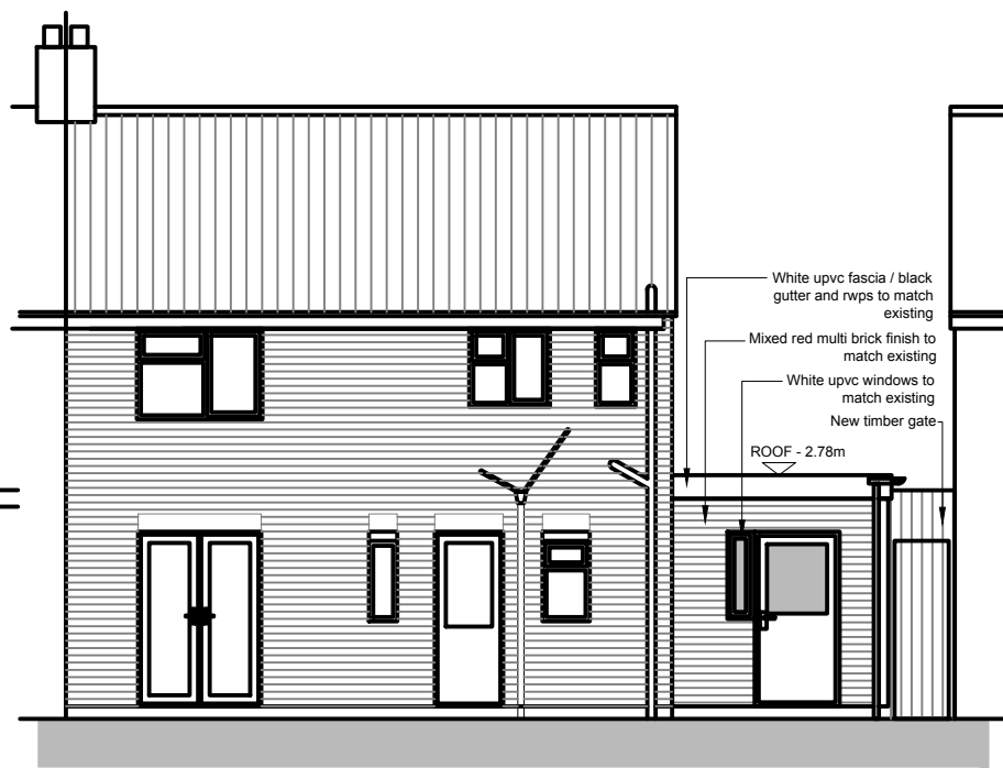
01 Proposed Rear Elevation 1:100 @ A3
