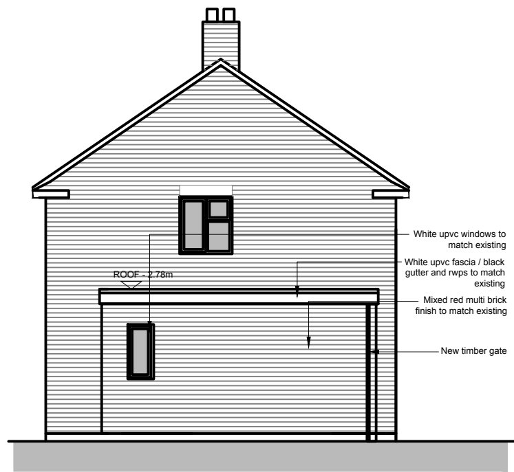
02 Proposed Side Elevation 1:100 @ A3
