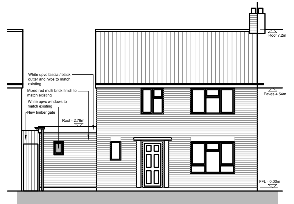
03 Proposed Front Elevation 1:100 @ A3
