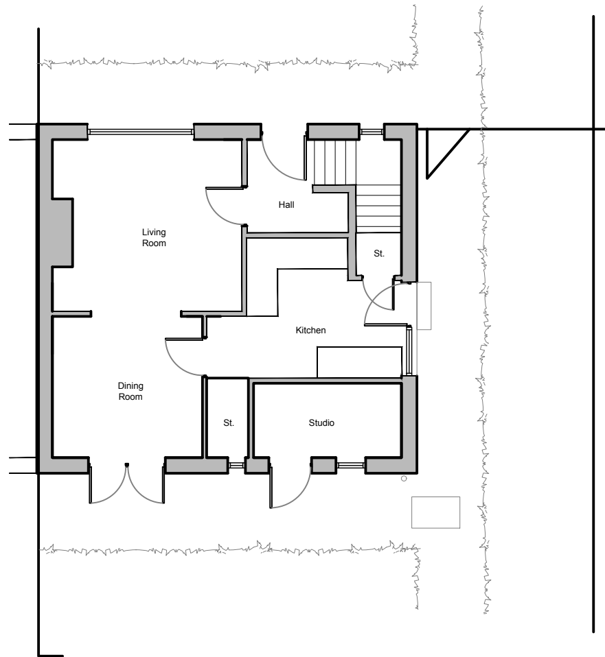
01 Existing Ground Floor Plan 1:100 @ A3
