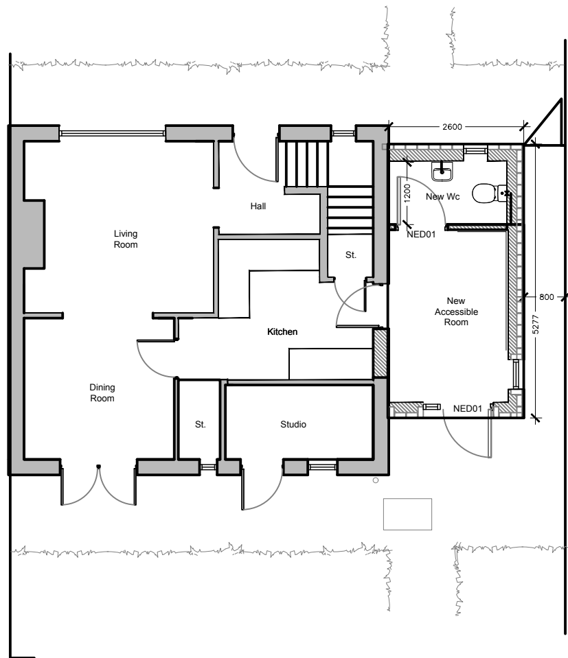
01 Proposed Ground Floor Plan 1:100 @ A3
