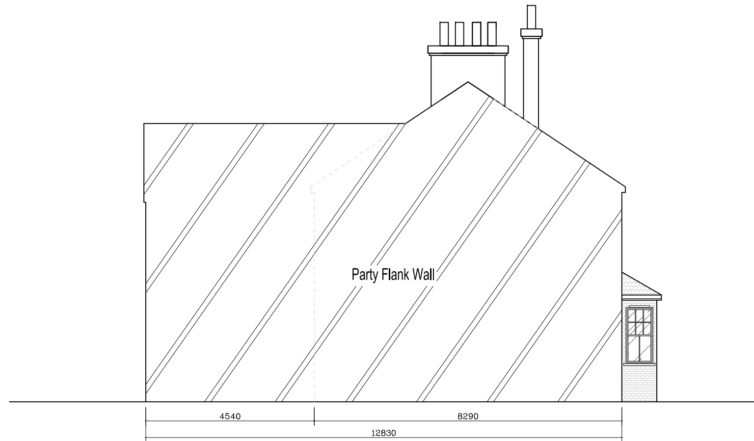
Existing Left Elevation 1-100 @ A3
