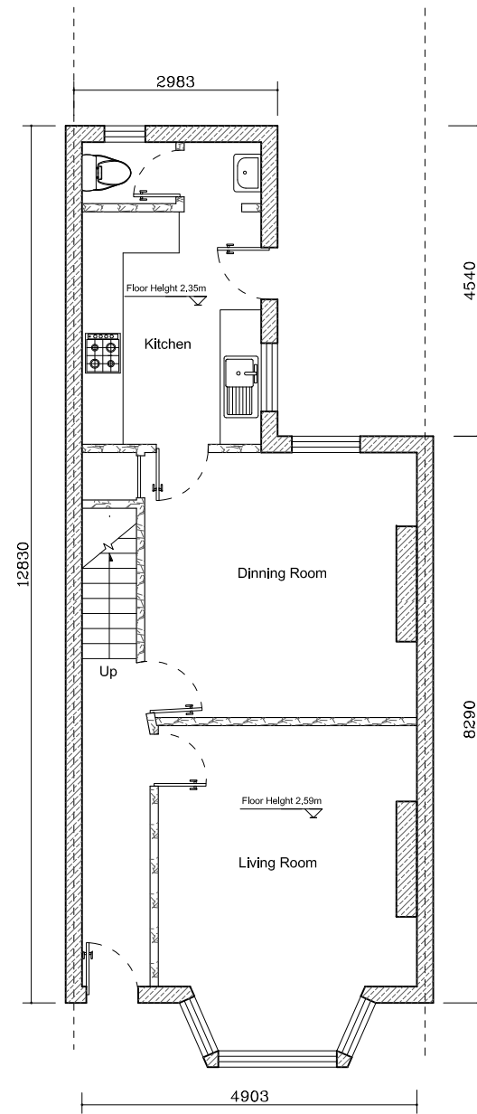
Proposed Ground Floor Plan 1-100 @ A3
