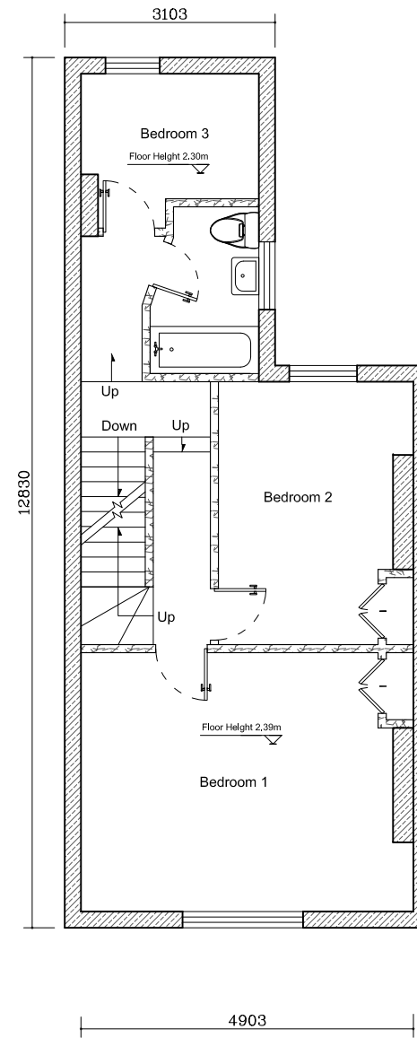
Proposed First Floor Plan 1-100 @ A3
