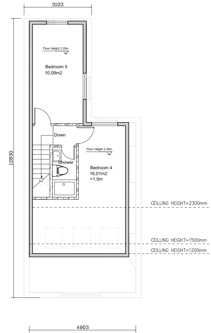
Proposed Second Floor Plan 1-100 @ A3
