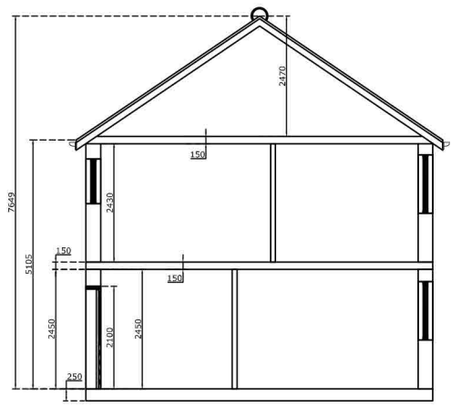
EXISTING SECTION A- A Scale 1:100@A3
