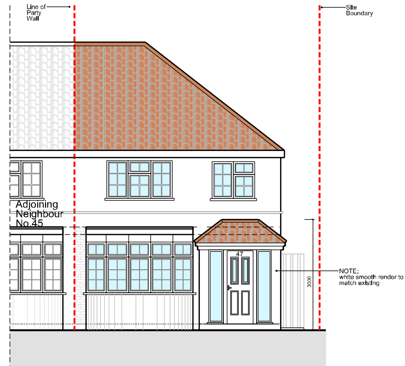
05 FRONT ELEVATION 1:100
