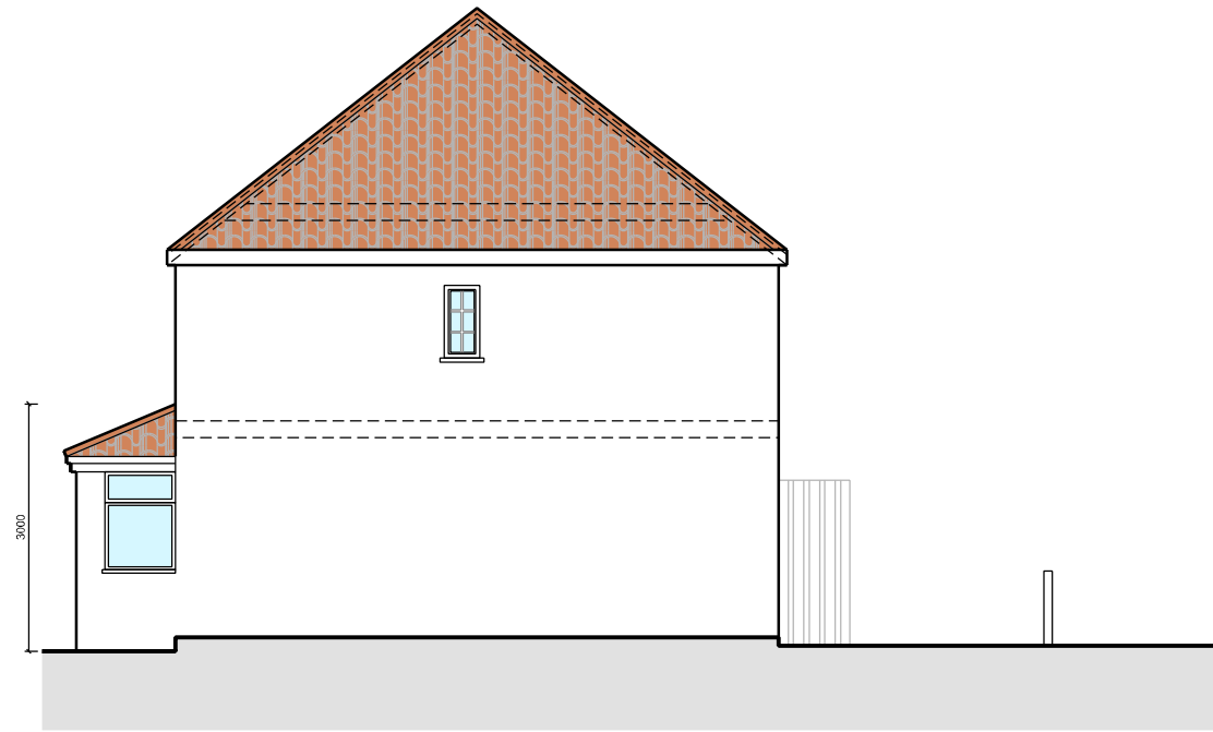
08 SIDE ELEVATION 1:100
