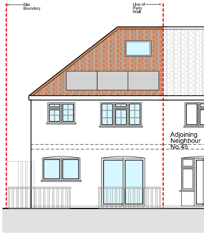
06 REAR ELEVATION 1:100
