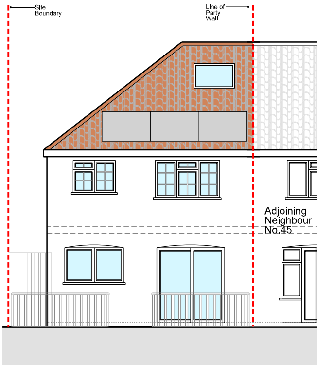
06 REAR ELEVATION 1:100
