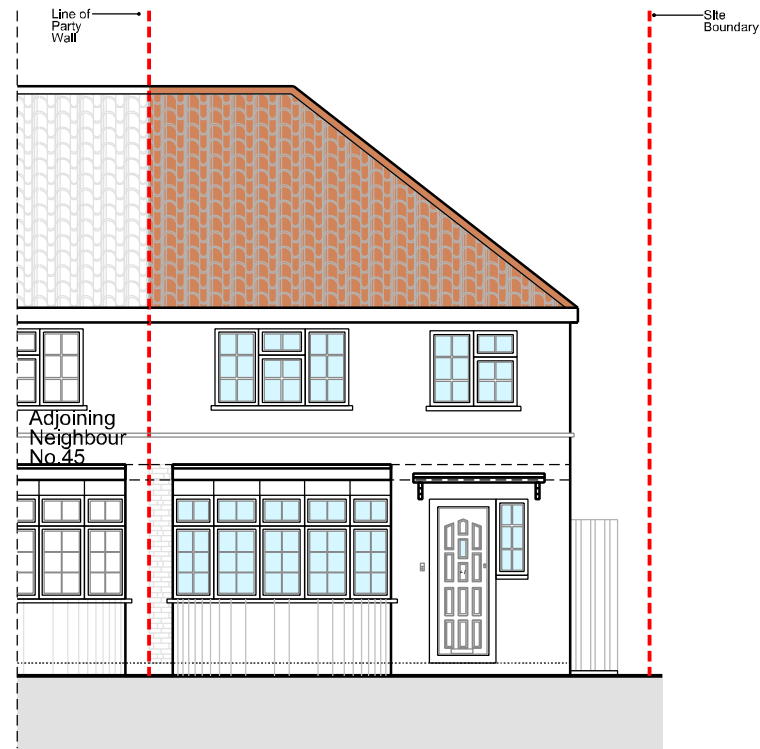
05 FRONT ELEVATION 1:100
