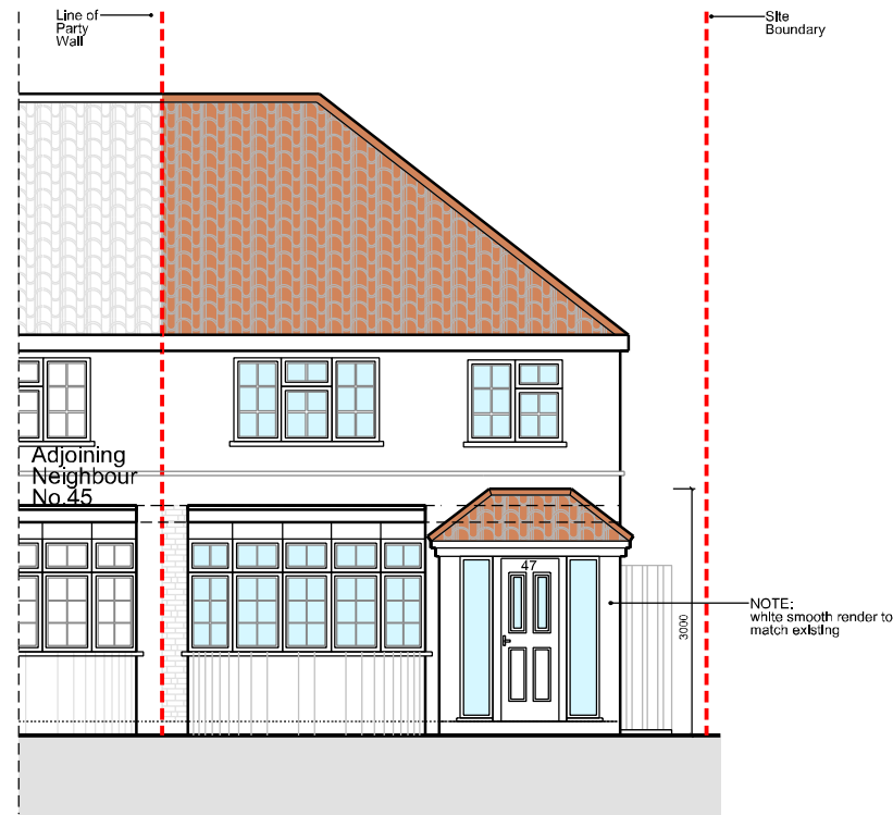
05 FRONT ELEVATION 1:100
