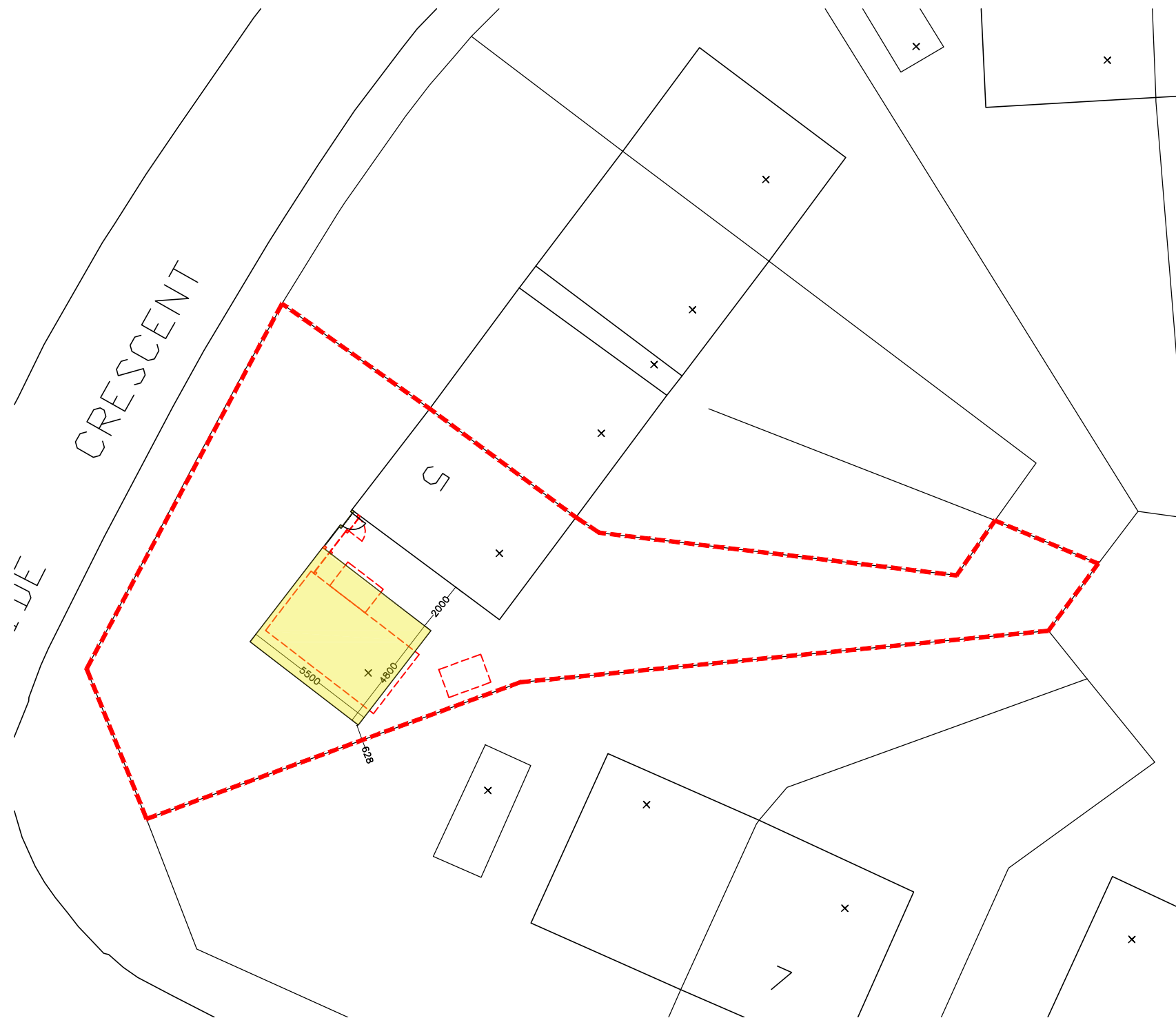
PROPOSED SITE PLAN SCALE 1:200.
