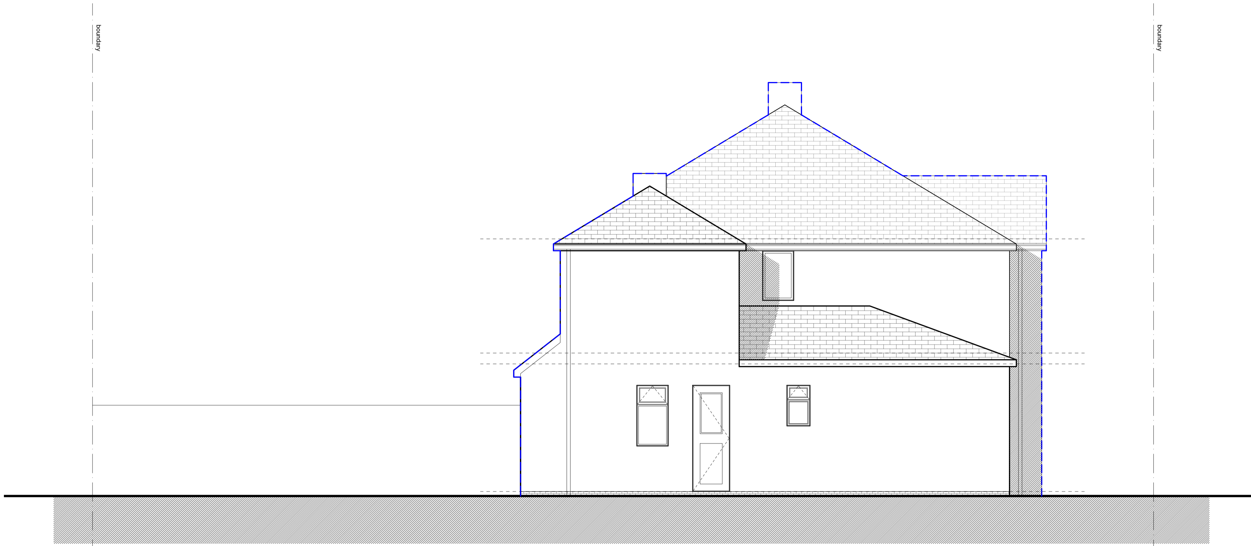
EXISTING SIDE ELEVATION A 1:50 Scale
