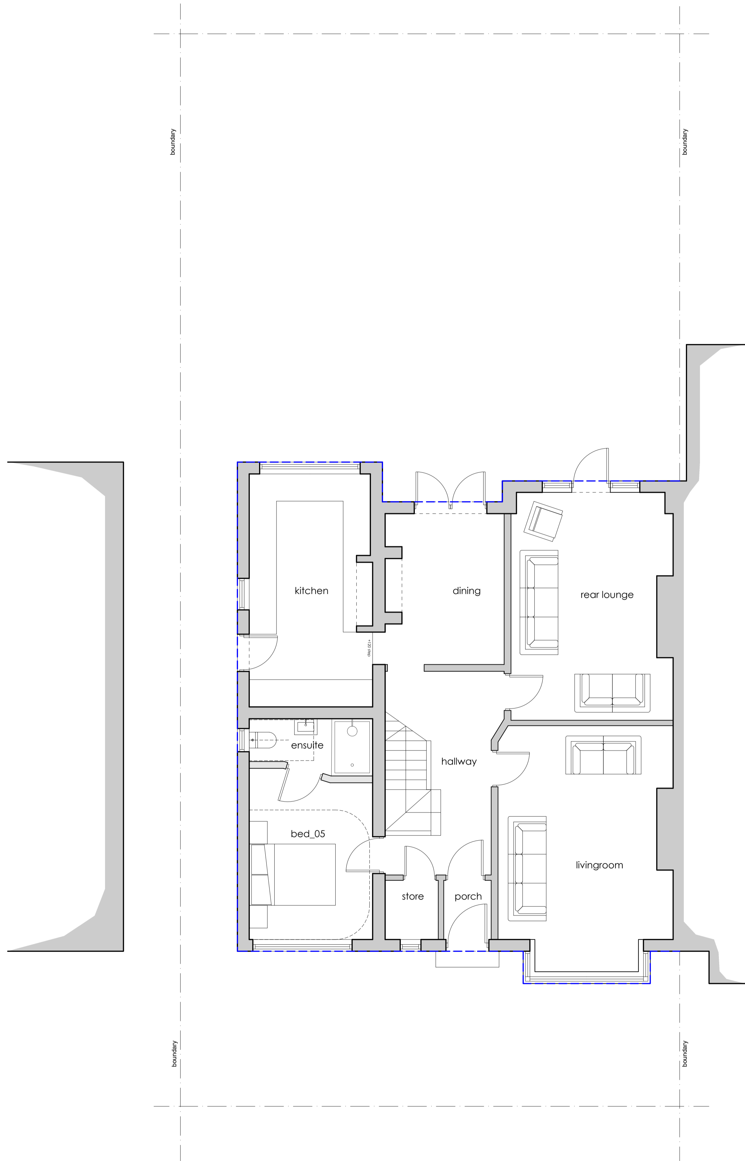
EXISTING GROUND FLOOR PLAN 1:50 Scale
