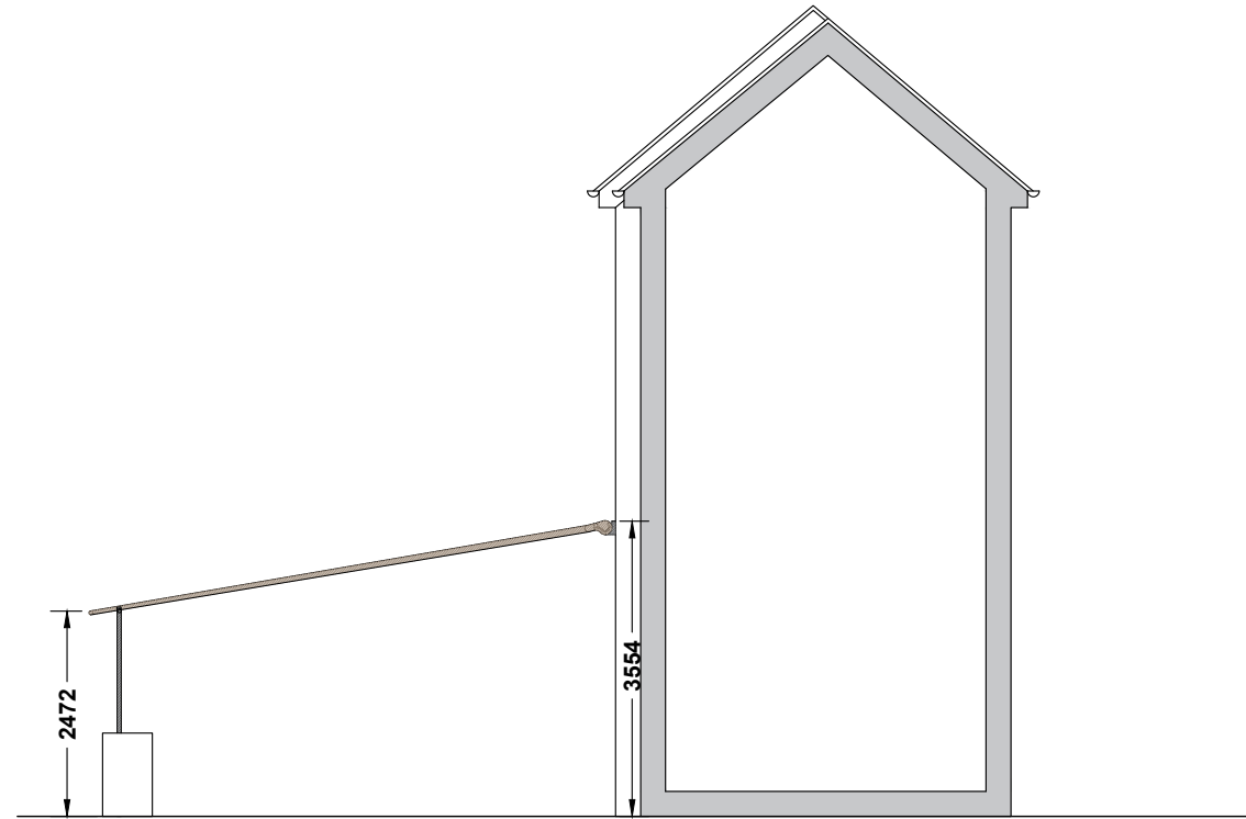
SIDE ELEVATION-NORTH EAST
