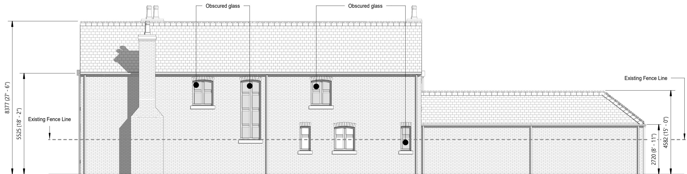
1 North Elevation 1 : 100
