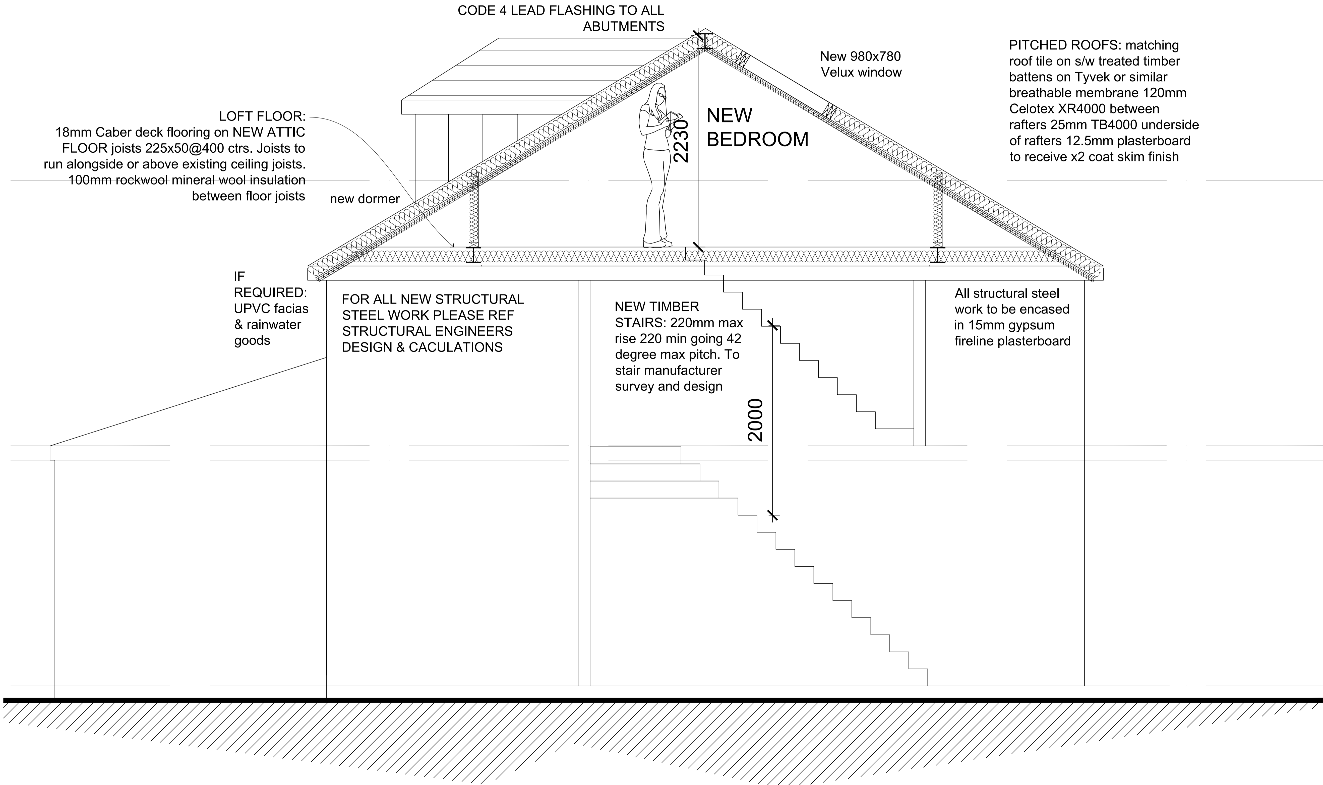
SECTION 1 - PROPOSED Scale - 1:20 @ A1
