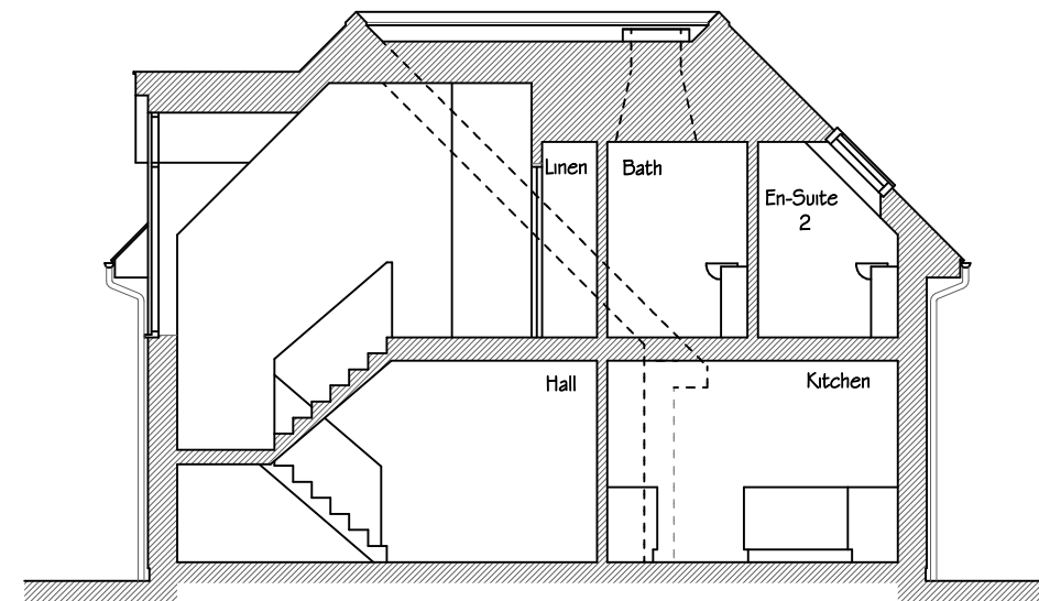
Cross Section
