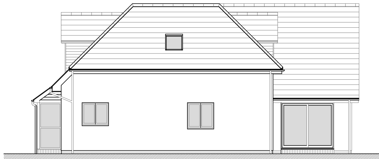
East Elevation
