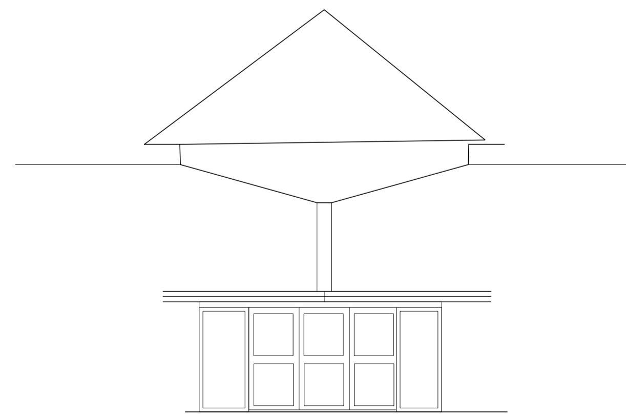
Entrance elevation
