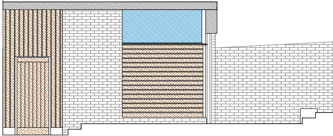
Side Elevation
