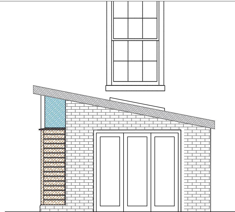
Rear Elevation
