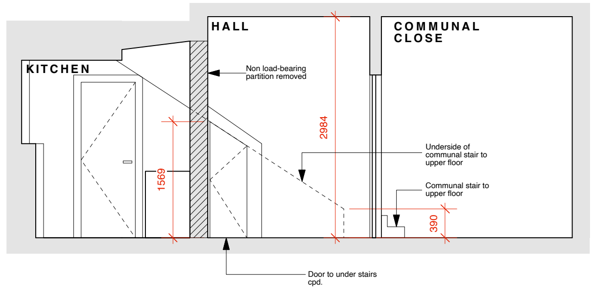
1 Existing Section AA 1:50
