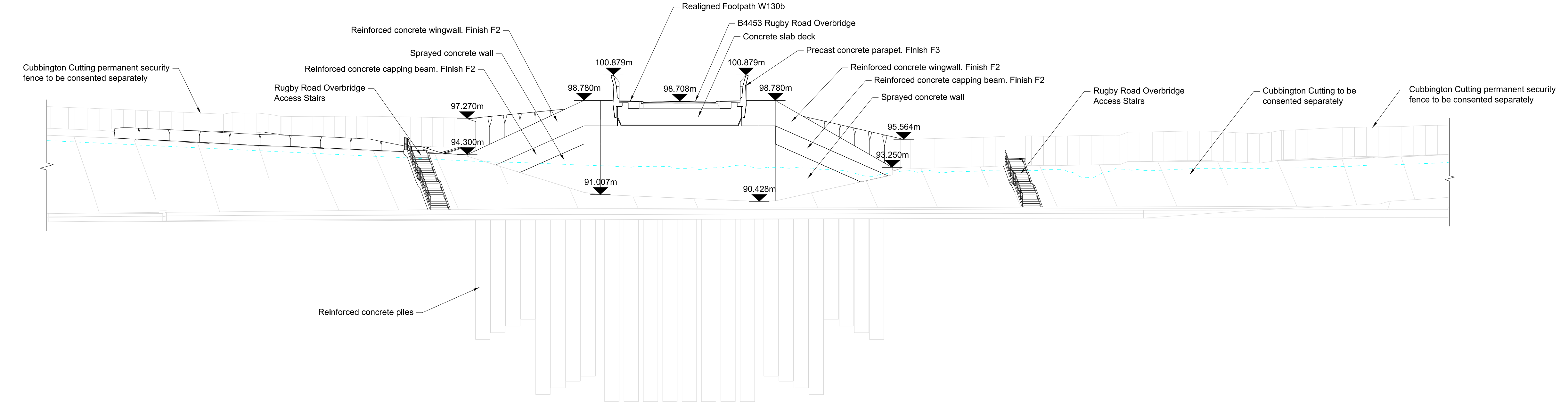
Section E Refer to Drawing No: 1MC08-BBV_MSD-PL-DGA-NS01_NL02-135602 Scale 1:200 @ A1
