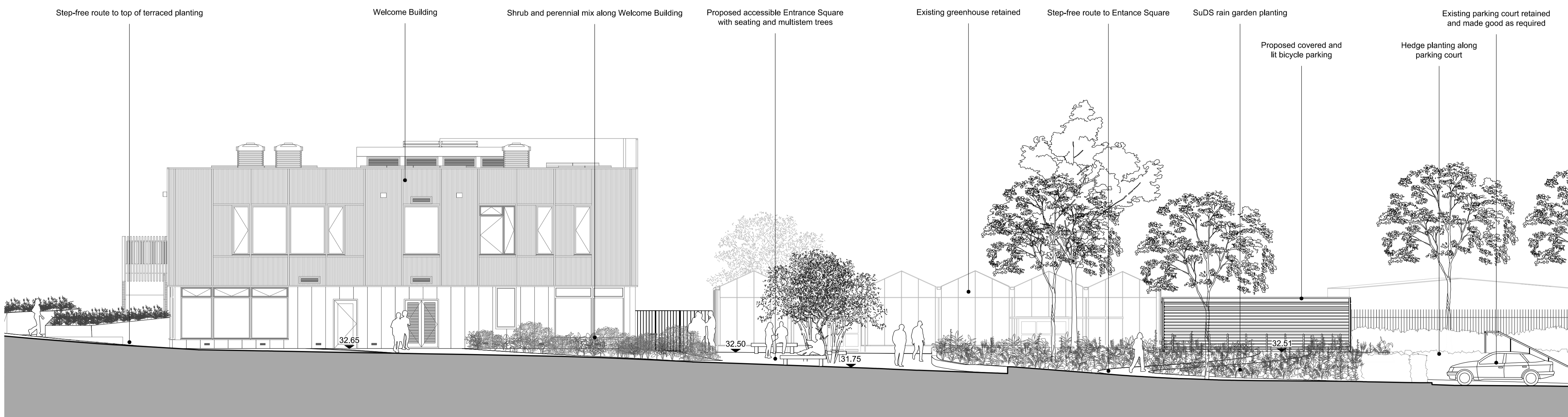
B-B' Proposed Section B-B' 1:100@A1
