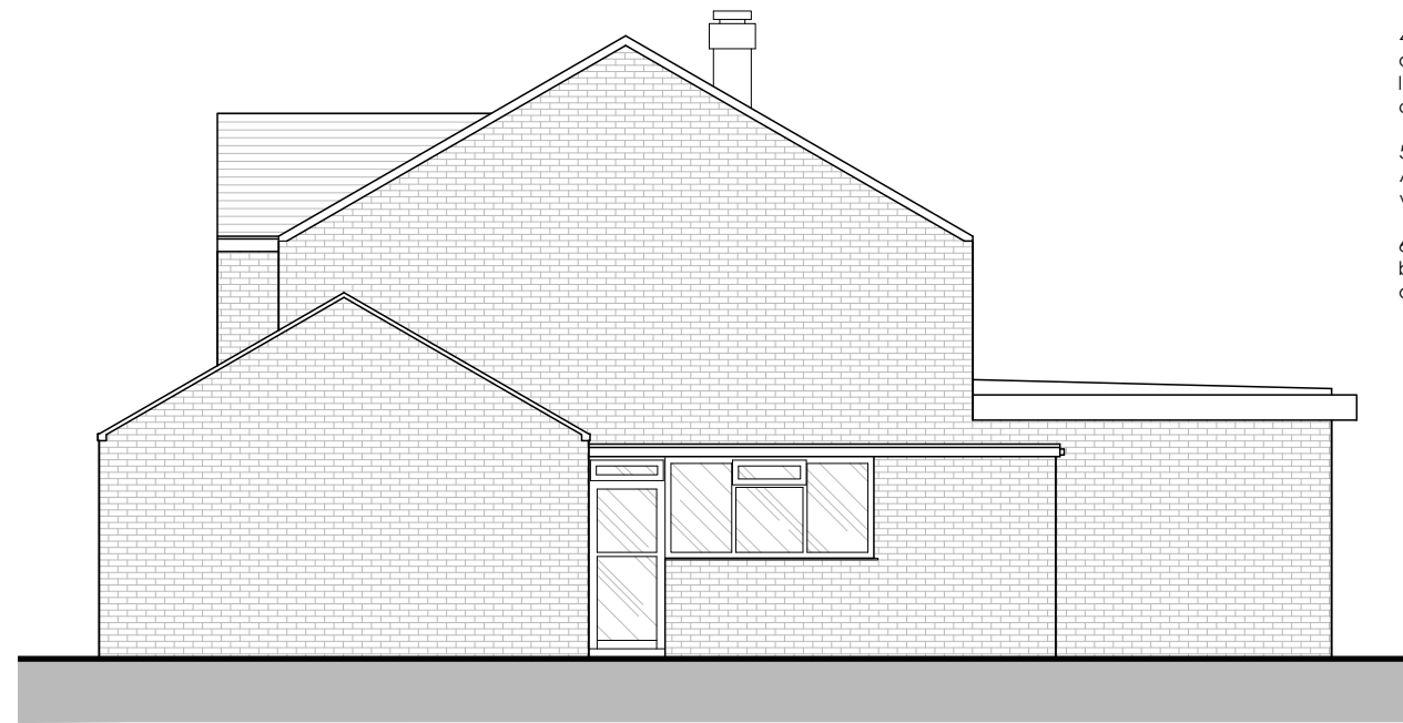
North Elevation - 1:100
