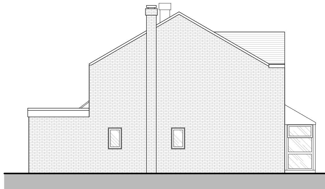
South Elevation - 1:100
