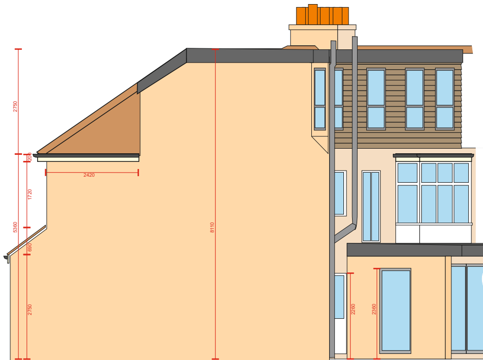
PROPOSED ELEVATION - VIEW FROM No.3
