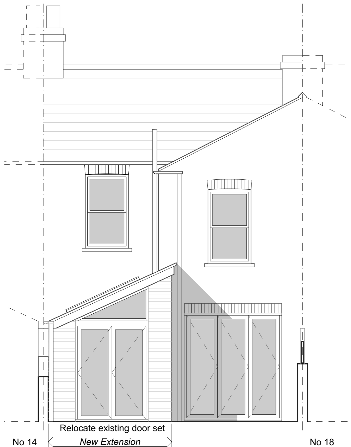
No 16 - Rear elevation - As Proposed
