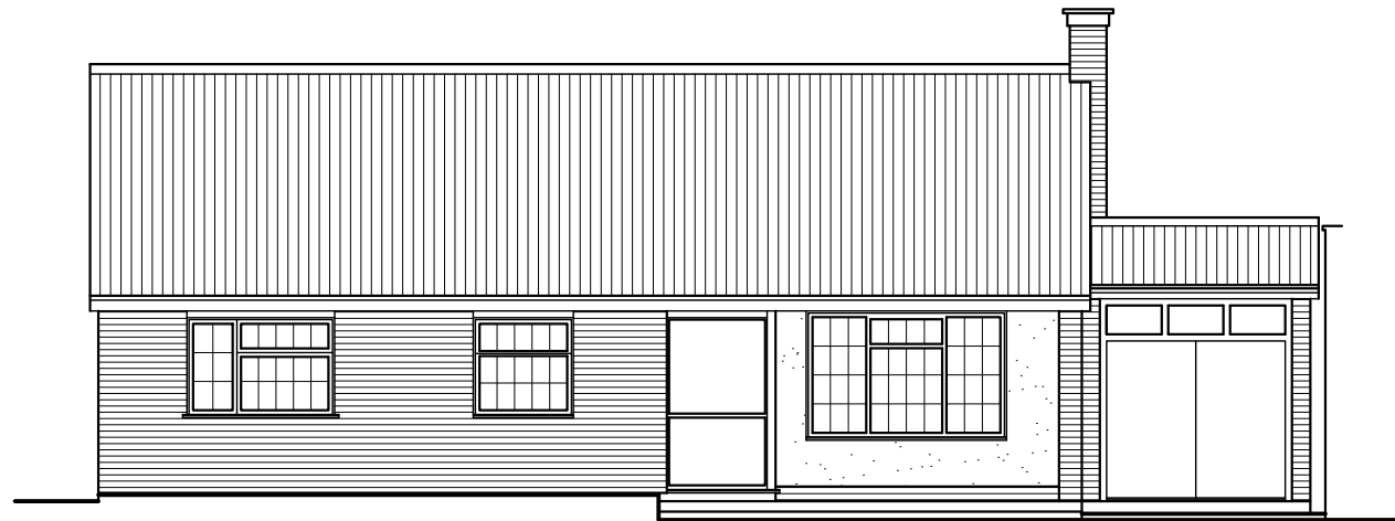
Existing Front Elevation - 1:100
