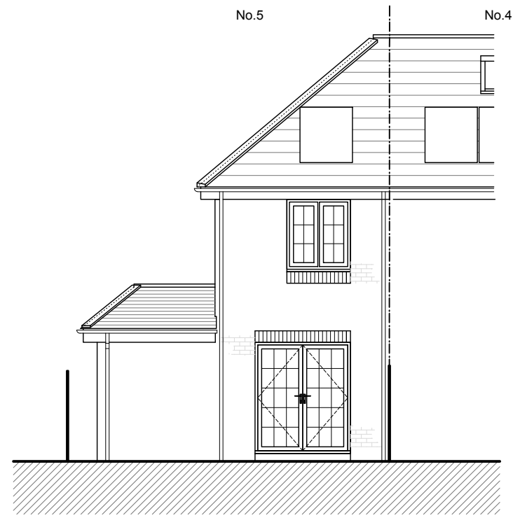
1 REAR ELEVATION 05
