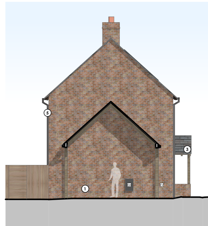
Plot 8 - Side (North/West) Elevation - Plot 8
