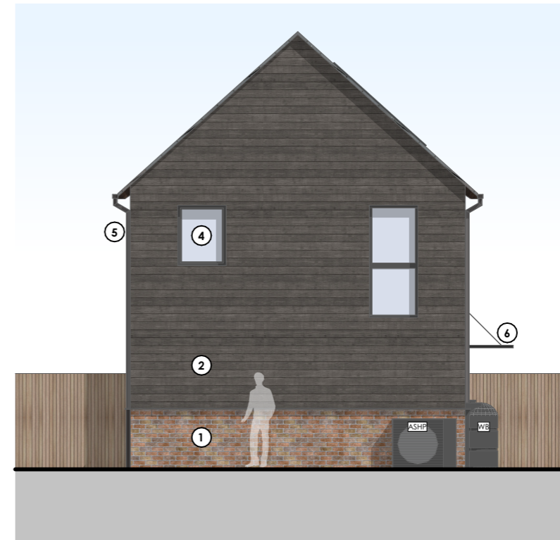
Plots 5/6 - Side (North/West) Elevation
