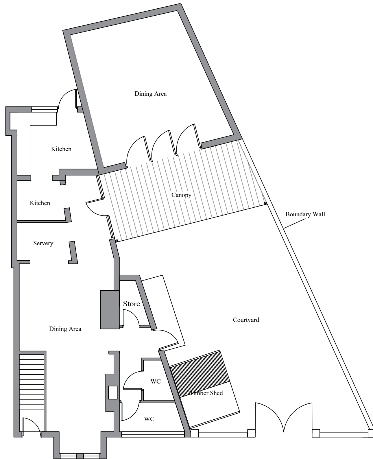
PROPOSED GROUND FLOOR LAYOUT PLAN
